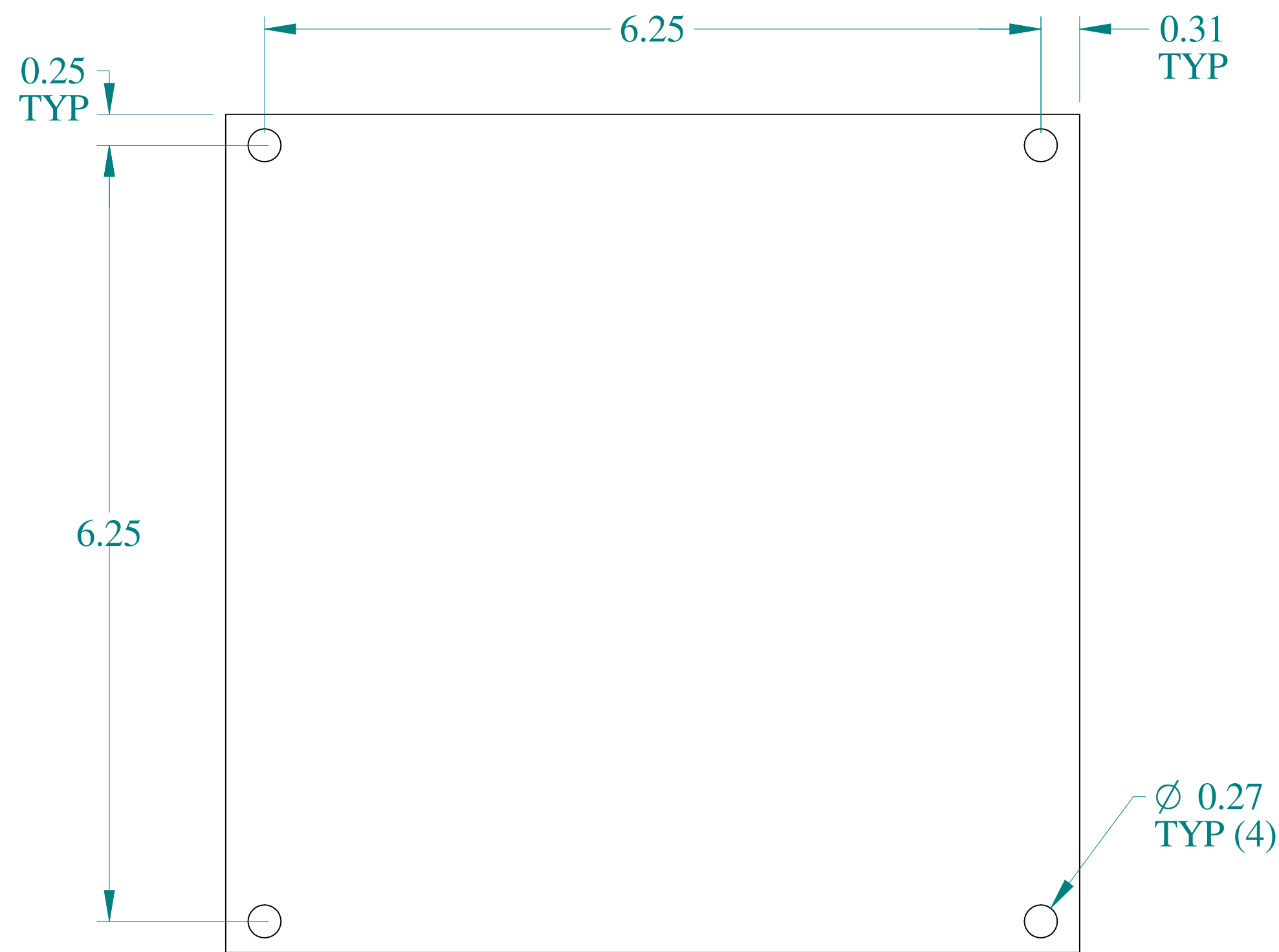
FRONT VIEW
