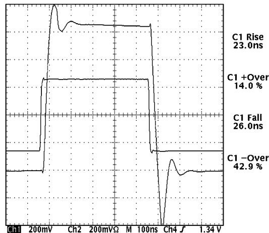
Figure 56. R_C = 240\Omega and C = 2.2 nF, Gain = +2
