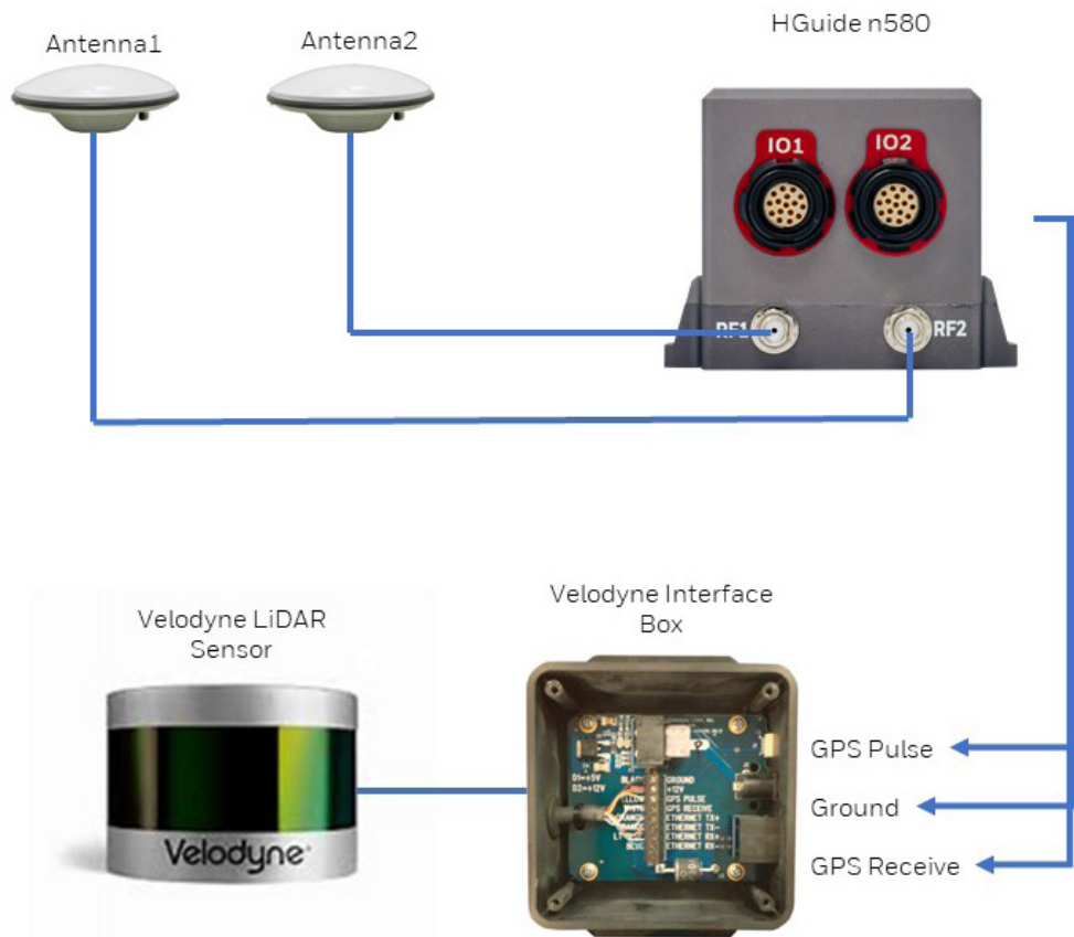
Figure 1: HGuide n580 -> LiDAR Interface Box -> LiDAR Diagram
