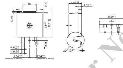
• No. 5 Surface-Mount (TO220S) MPL-102S, MP2-202S, MPL-1036
