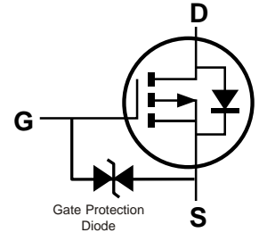
Internal Schematic
