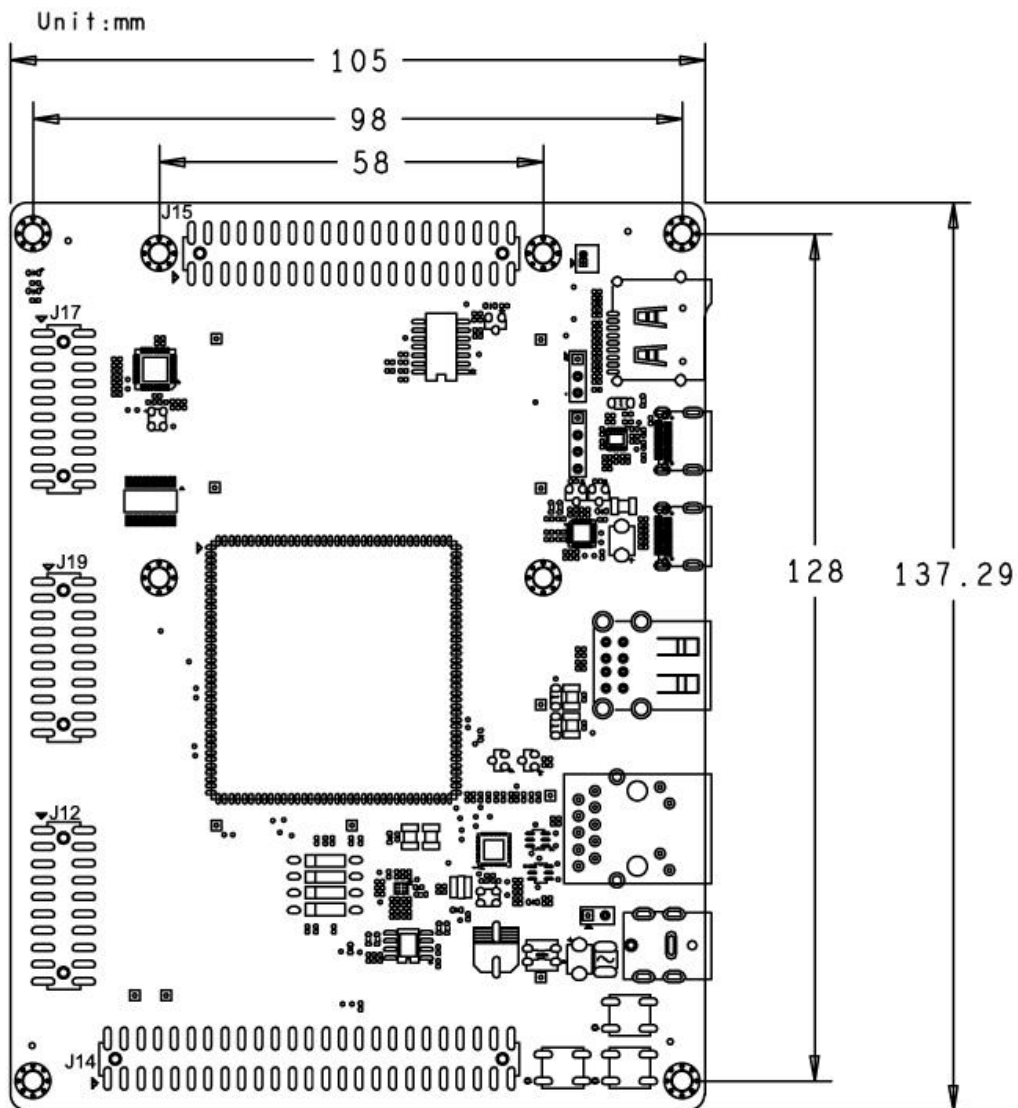
Figure 1-10 MYD-YA15XC-T Dimensions Chart
