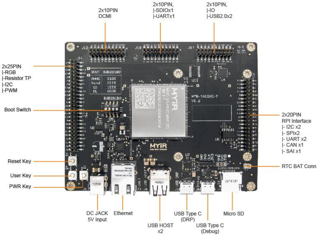
Figure 1-2 MYD-YA15XC-T Development Board Top-view
