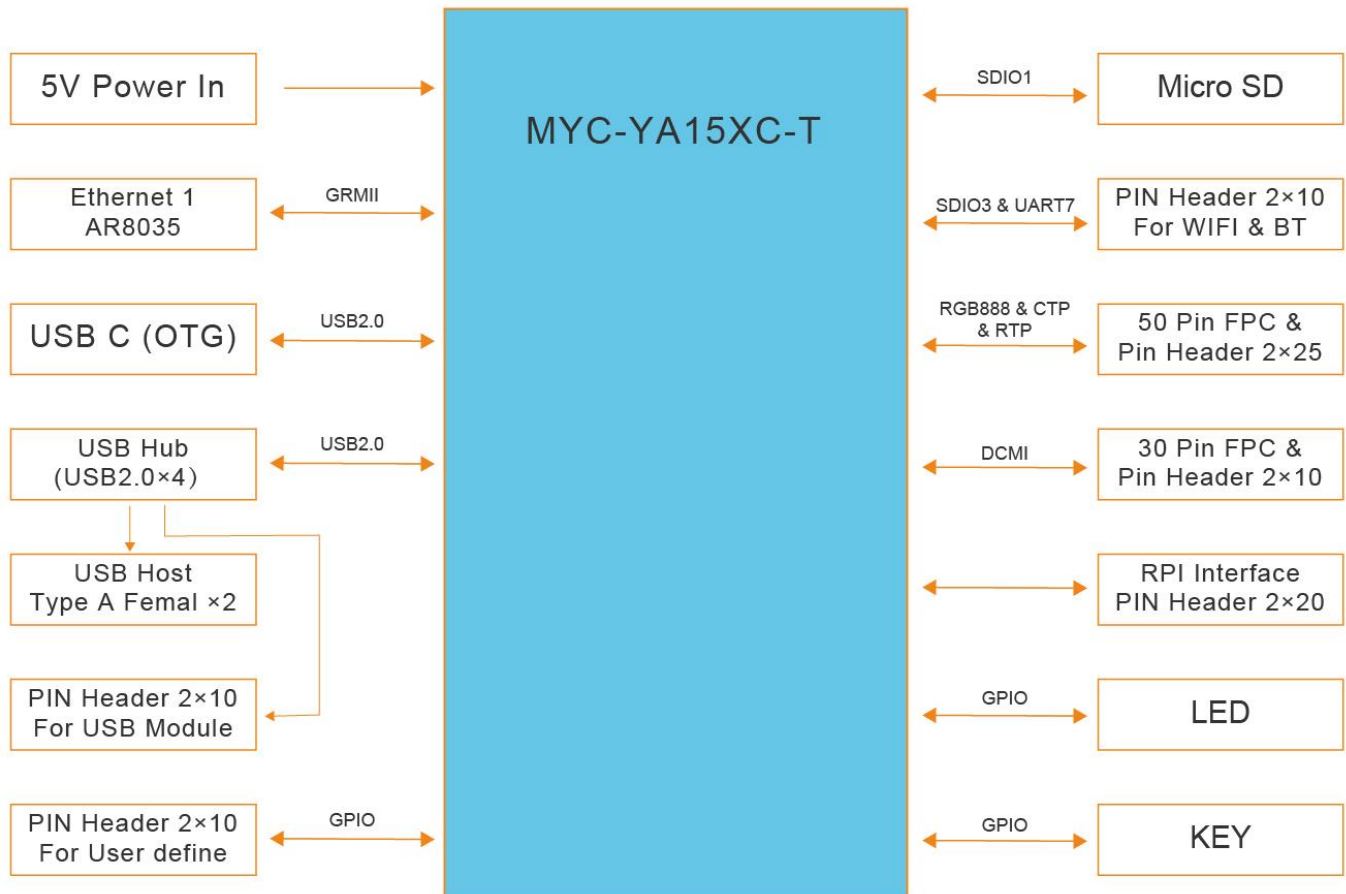
Figure 1-8 MYD-YA15XC-T Development Board Function Block Diagram
