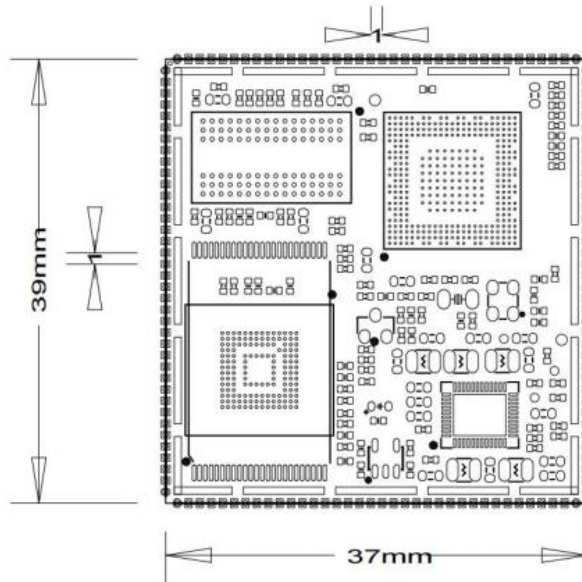
Figure 1-9 MYC-YA15XC-T Dimensions Chart
