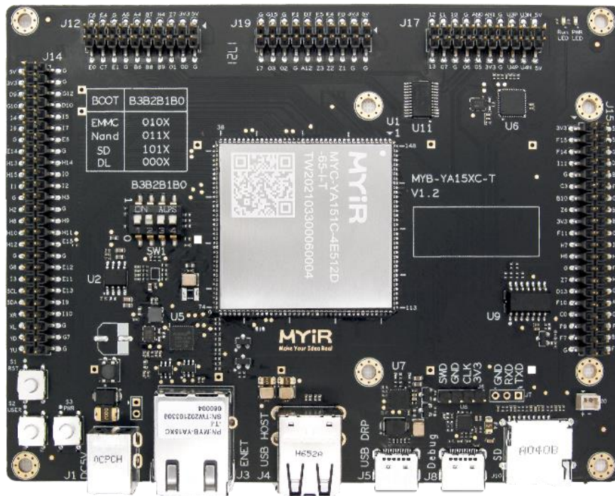
Figure 1-1 MYD-YA15XC-T Development Board
