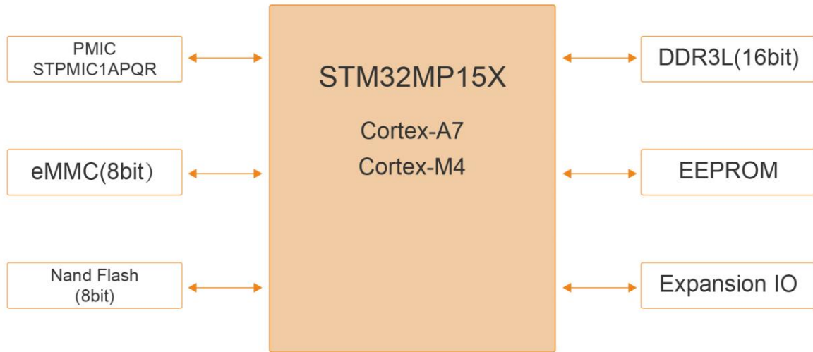
Figure 1-7 MYC-YA15XC-T CPU Module Function Block Diagram
