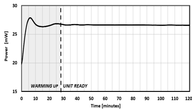
FIG. 13: WARM-UP TIME
