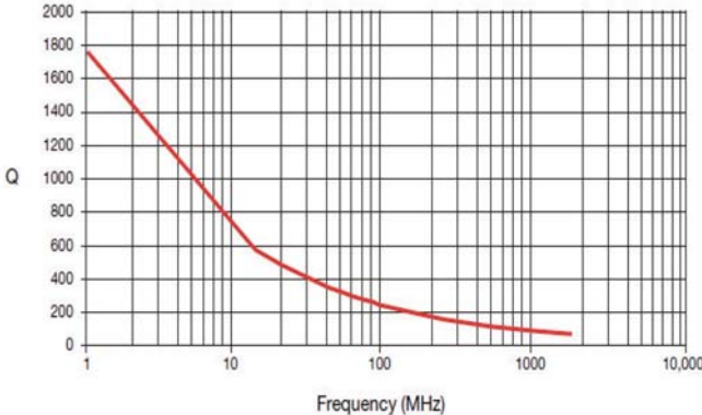
22pF Q vs. Frequency
