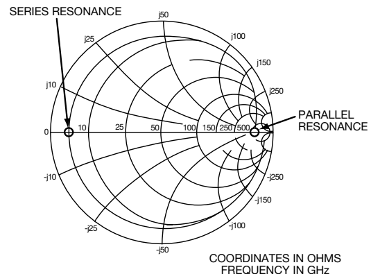
Figure 10. SLC Impedance on Smith Chart
