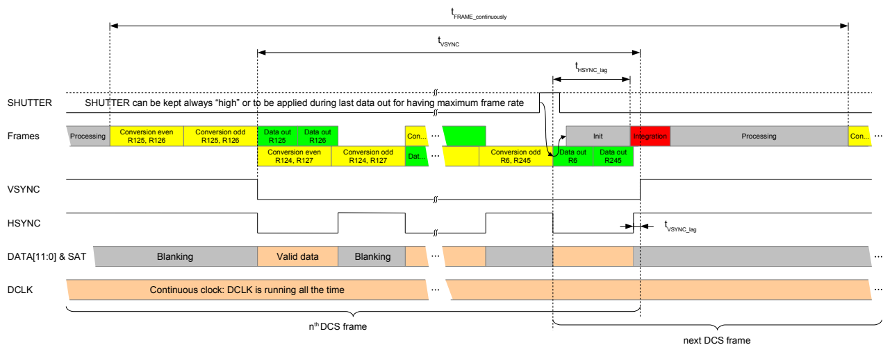
Figure 29: Frame timing: Inter frame timing, end of frame and start next frame
