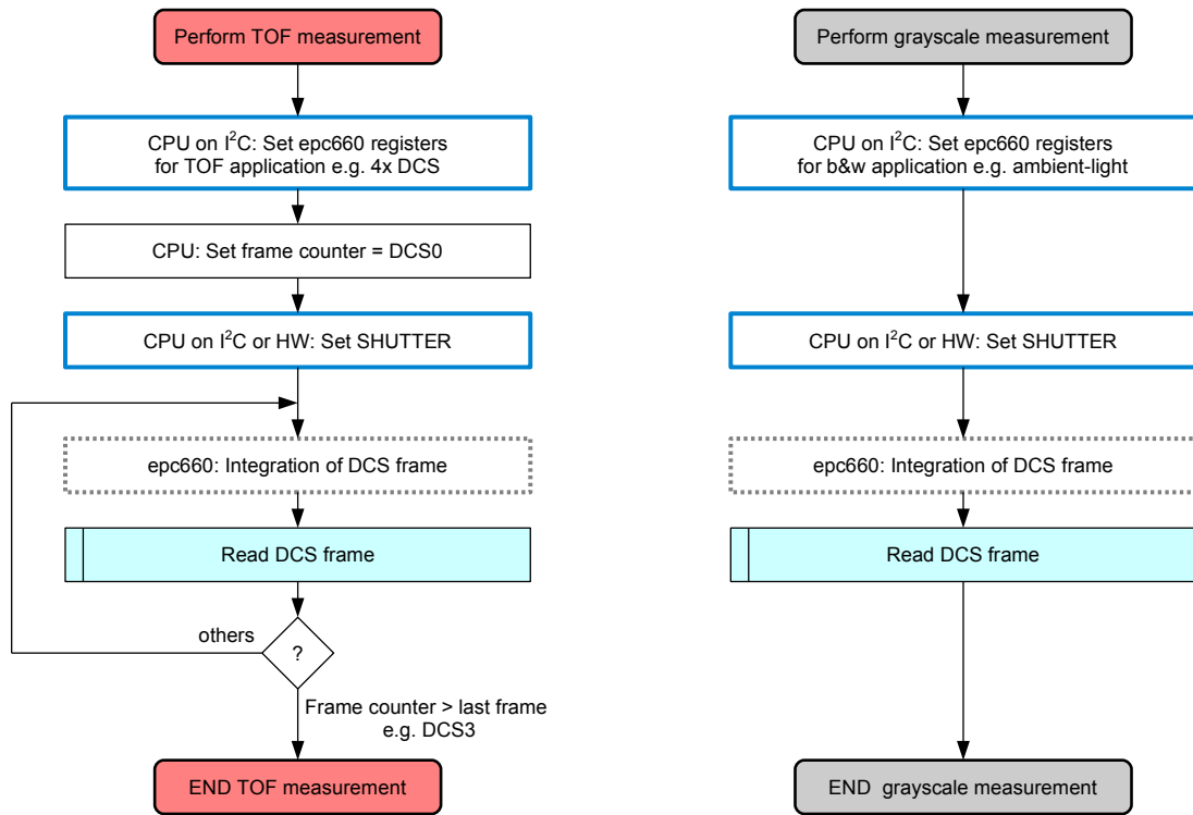
Figure 54: Generic sequences for the distance (TOF) and the grayscale measurement
