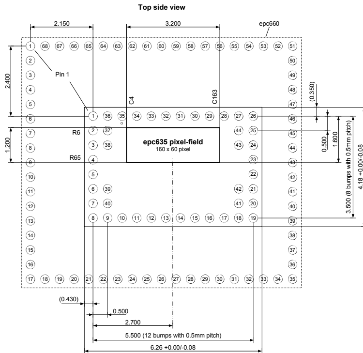
Figure 58: Mechanical dimensions epc635 versus epc660, pin 1
