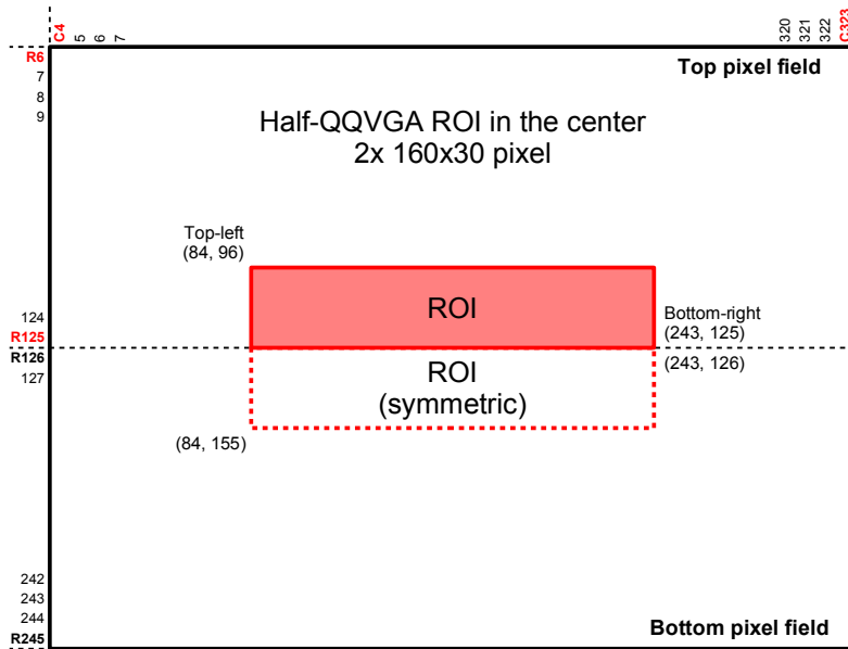
Figure 34: ROI for Half-QQVGA: 2 x 160 x 30 pixel
