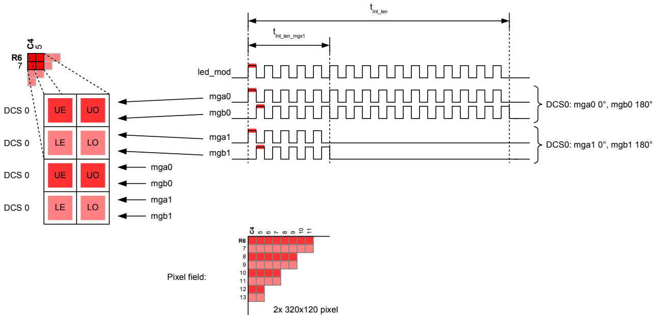
Figure 39: Dual integration time mode: even and odd rows independently controlled by mgx0 and mgx1. One stops earlier than the other.
