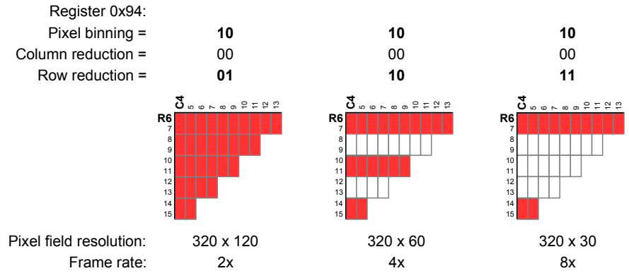
Figure 43: Row reduction on y-axis combined with vertical binning
