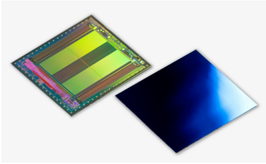
Figure 14: epc660-CSP68 bottom and top side
