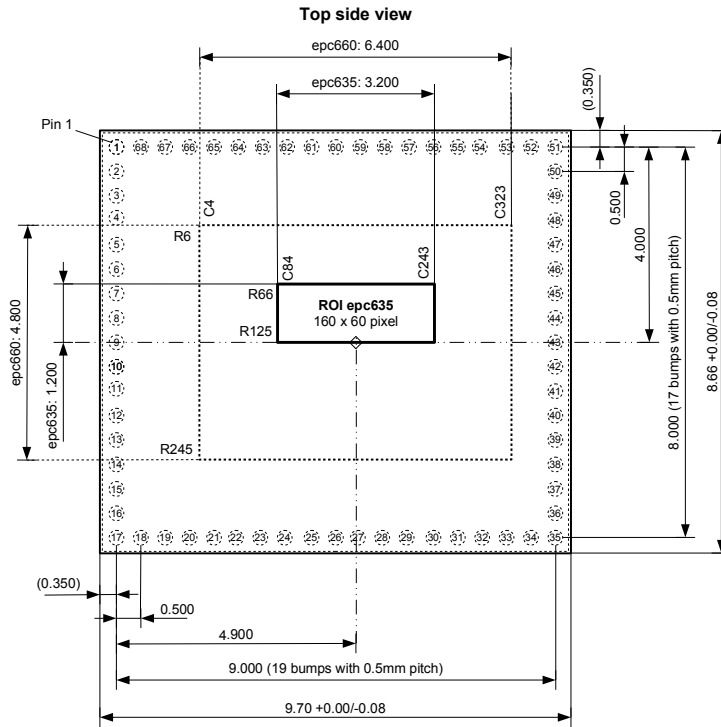
Figure 57: epc660: ROI setting for epc635 emulation
