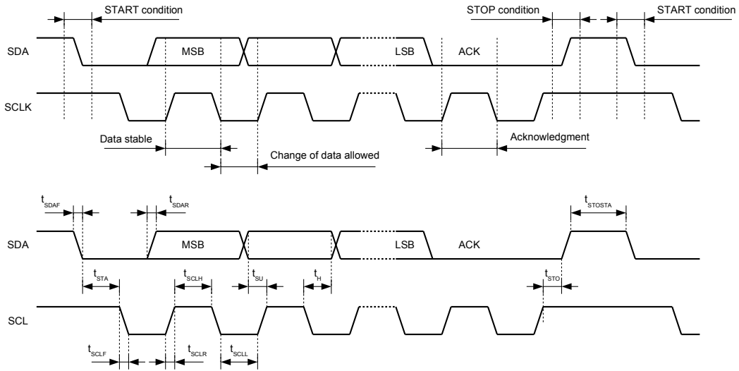
Figure 64: I 2 C bus timing
