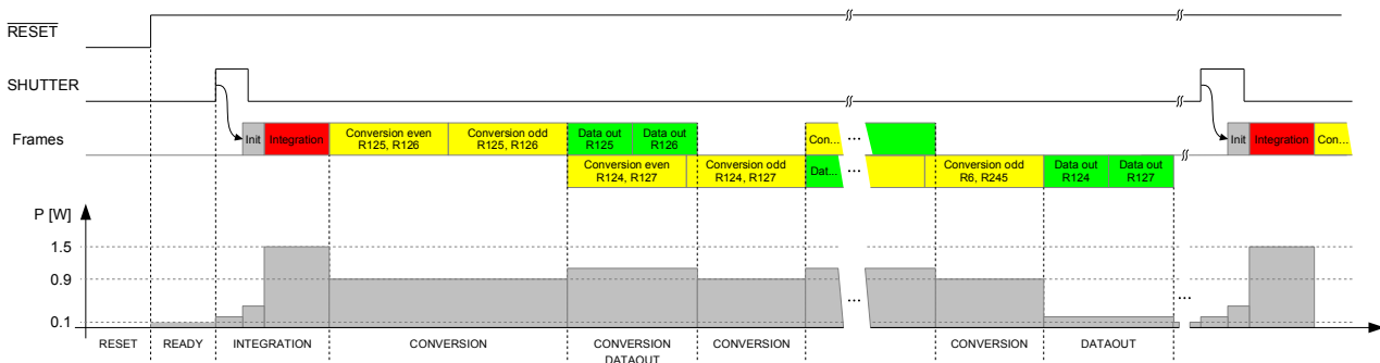
Figure 59: Power consumption levels and operating states
