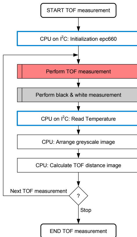
Figure 53: Generic 3D TOF distance measurement flow
