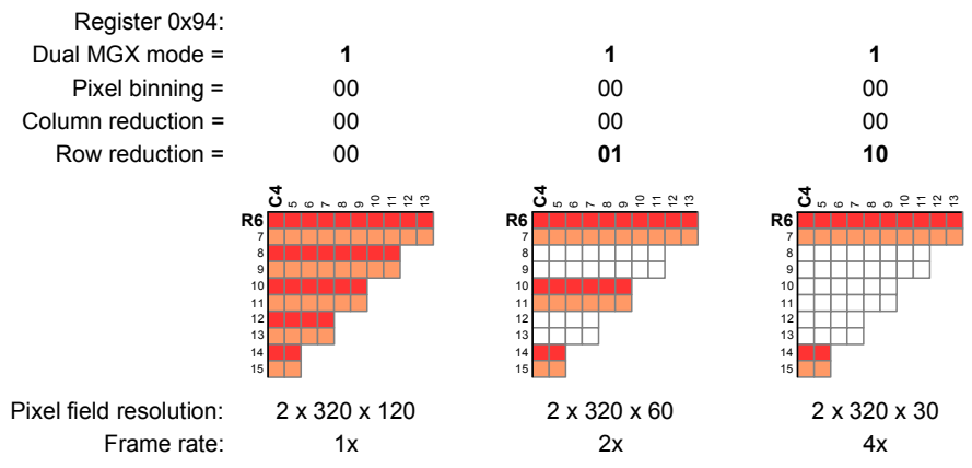
Figure 45: Row reduction on y-axis combined dual phase mode
