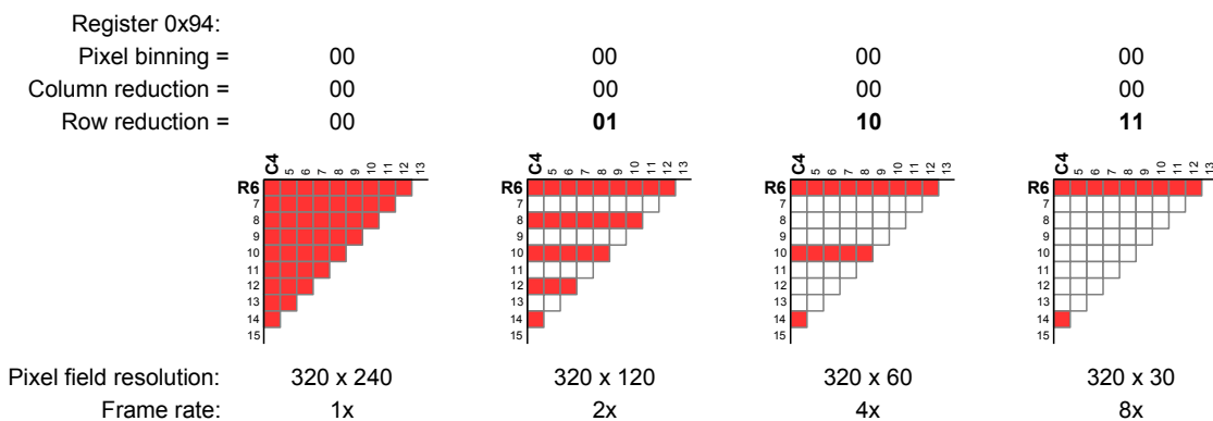
Figure 41: Row reduction on y-axis without binning
