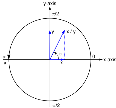
Figure 50: Continuous atan2 representation for the range -\pi \dots +\pi
