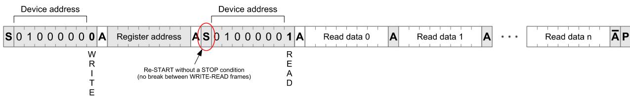
Figure 70: Multi-byte Read access through I 2 C
