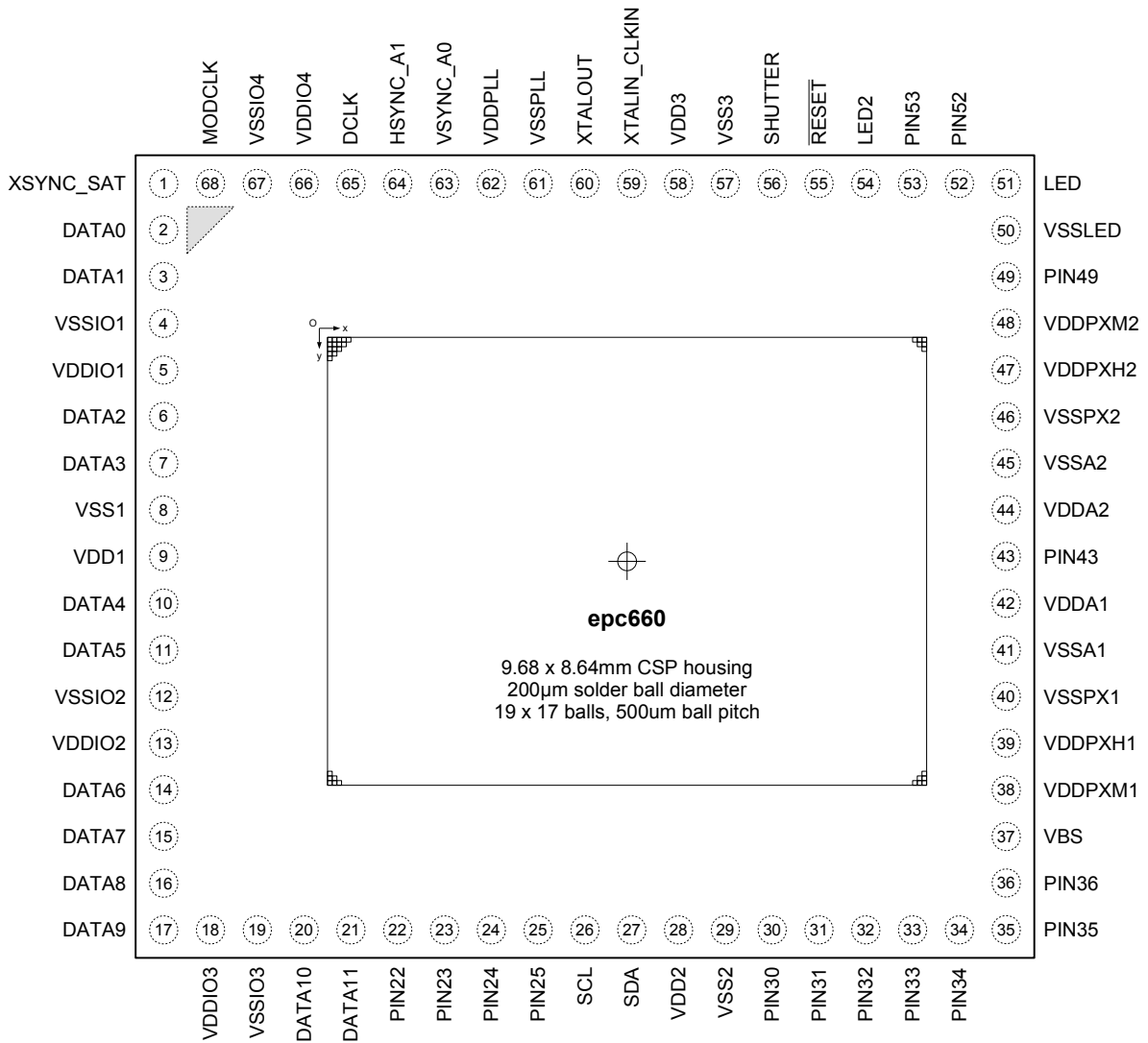
Figure 7: CSP pin mapping (top-view, solder balls are at the bottom, pixel-field is at the top)
