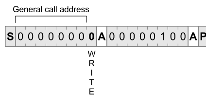
Figure 66: Device address A1, A0 reload through I 2 C
