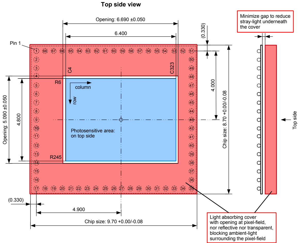
Figure 10: Opaque cover for protection against unwanted ambient-light
