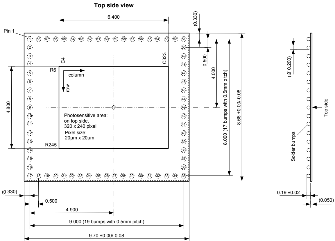
Figure 9: Mechanical dimensions
