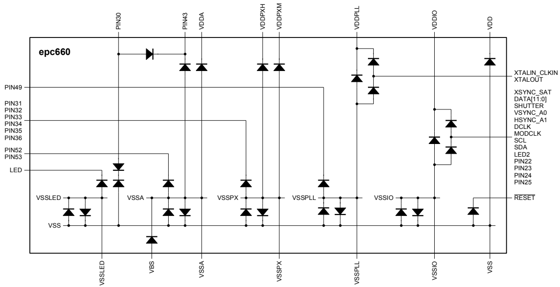
Figure 8: I/O pins and ESD protection diagram
