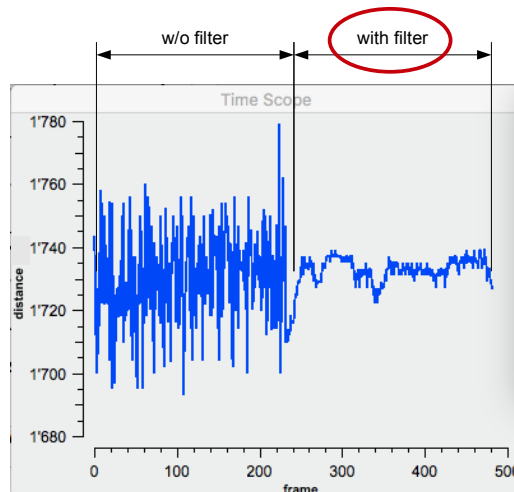
Figure 52: Effect of the static Kalman filter on distance noise (Distance in mm)
