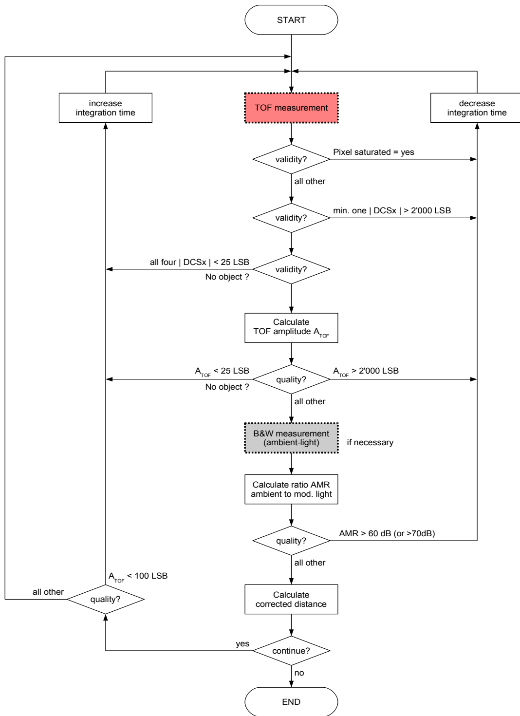
Figure 56: Generic validity and quality flow chart for a single pixel
