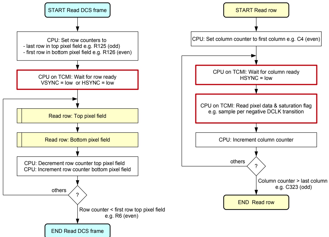
Figure 55: Generic sequences to readout frames and row by row
