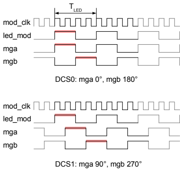
Figure 48: 4 DCS modulation/demodulation waveforms
