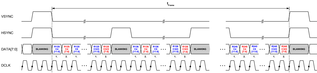
Figure 31: msb/lsb split mode
