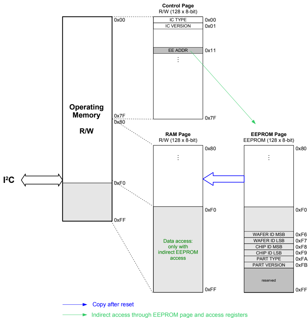
Figure 62: Memory map
