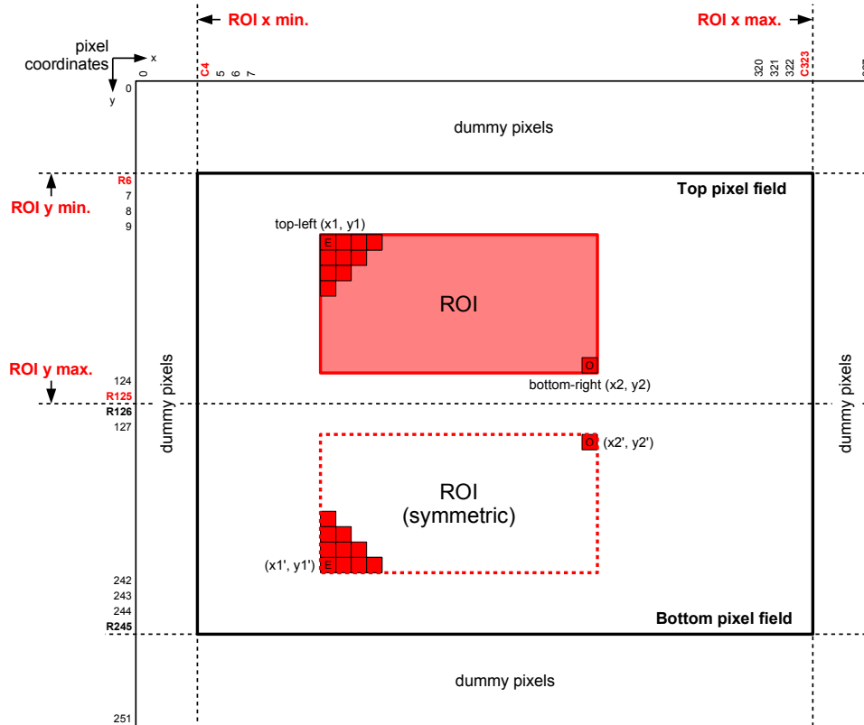
Figure 47: Region of interest (ROI)
