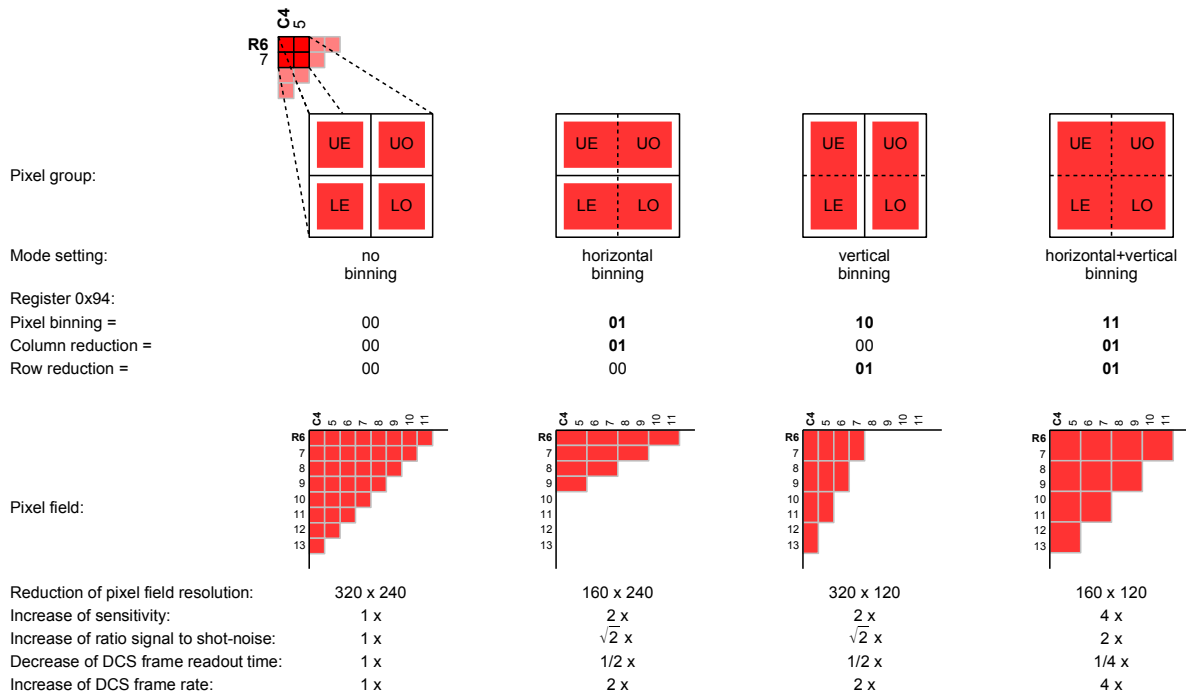
Figure 40: Pixel binning modes and readout
