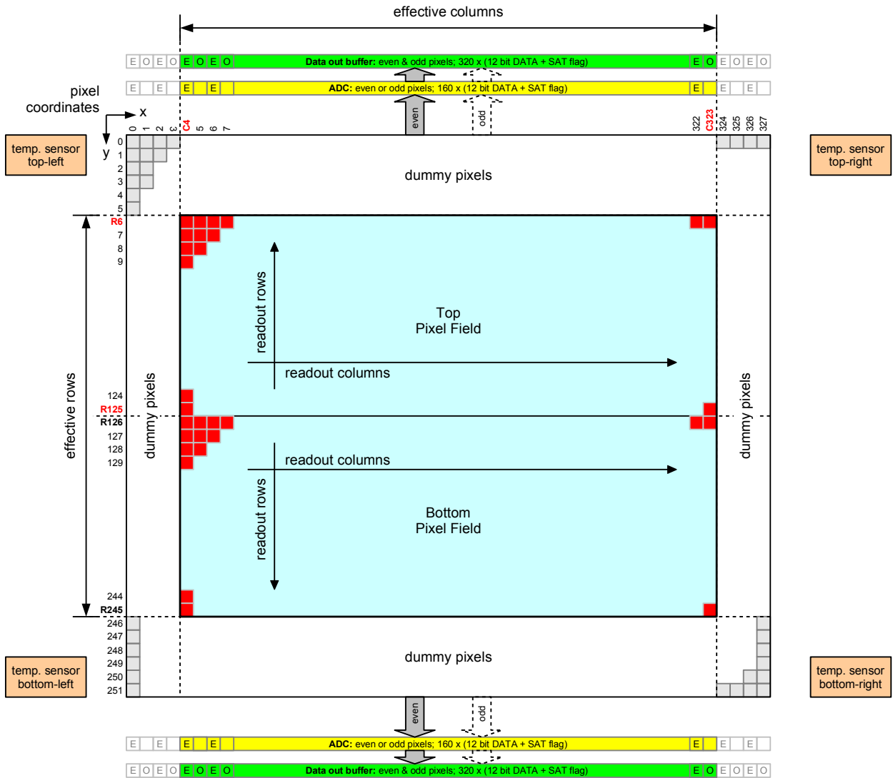
Figure 36: Pixel-field coordinates with row and column numbering scheme (top-view, solder balls are bottom side)
