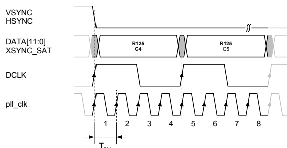
TCMI detailed bus timing: DCLK=24MHz ( pll\_clk / 4 )
