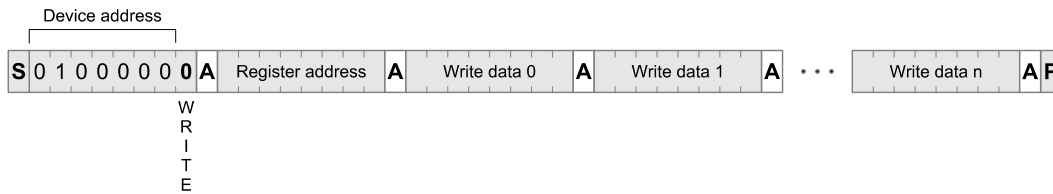
Figure 68: Multi-byte Write access through I 2 C
