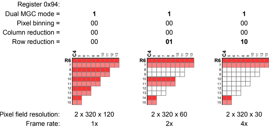
Figure 46: Row reduction on y-axis combined with dual integration time mode.
