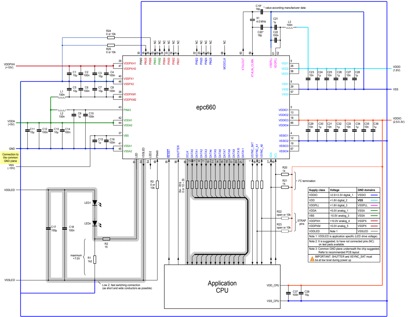
Figure 16: Typical application diagram
