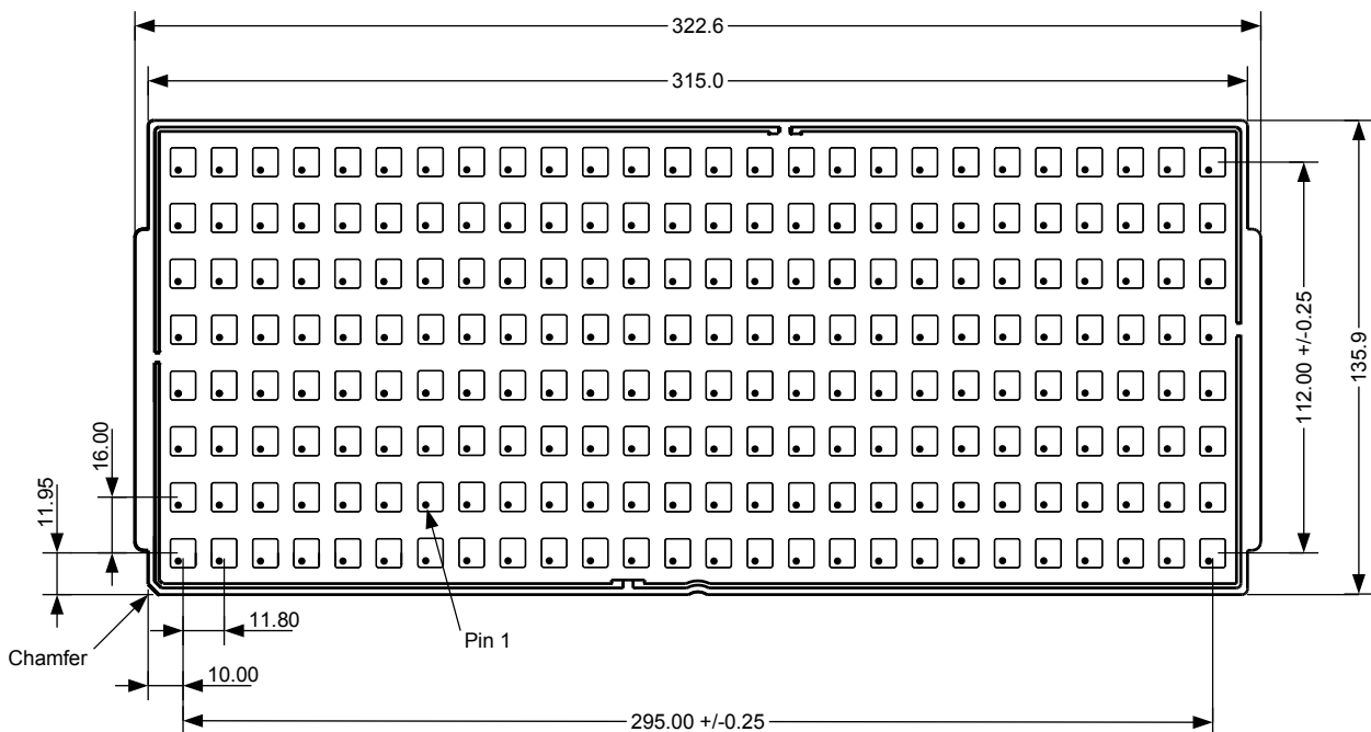
Figure 13: JEDEC tray for 26 x 8 pieces, maximum quantity 208 pieces per tray, use vacuum pick-up (all measures in mm)
