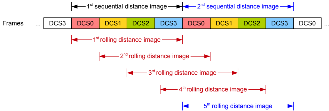
Figure 60: Rolling DCS frames
