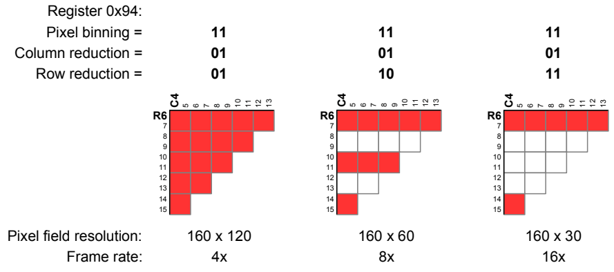
Figure 44: Row reduction on y-axis combined with horizontal and vertical binning
