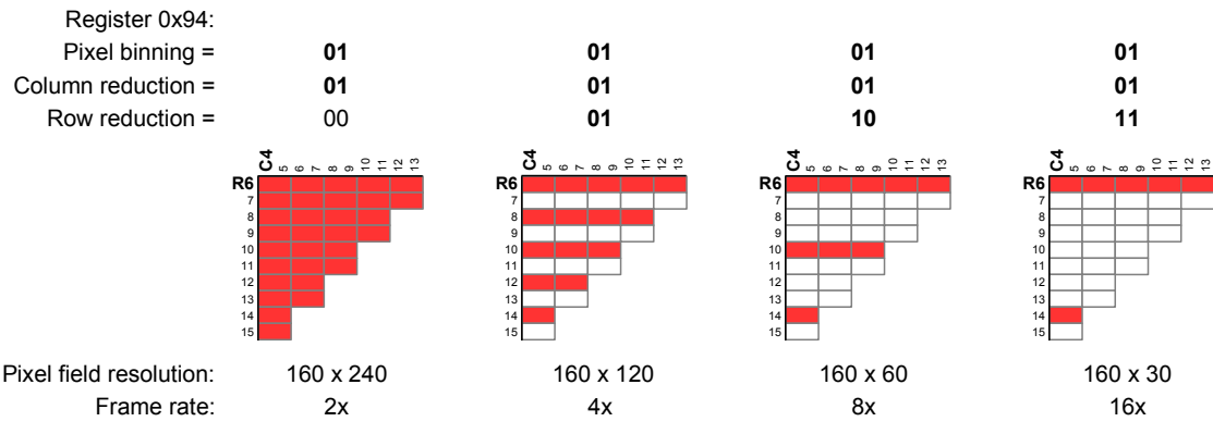
Figure 42: Row reduction on y-axis combined with horizontal binning
