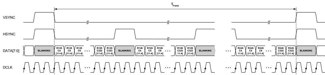
Figure 33: 8-bit mode
