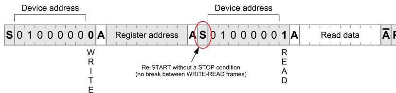
Figure 69: Single-byte Read access through I 2 C
