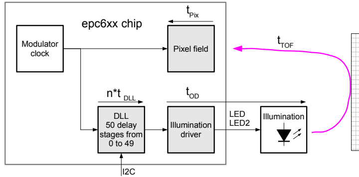
Figure 21: Block diagram of the DLL function
