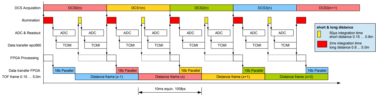
Figure 61: Enhanced rolling mode sequence
