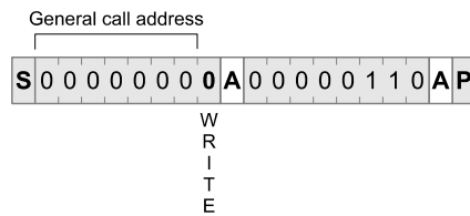
Figure 65: Software reset through I 2 C
