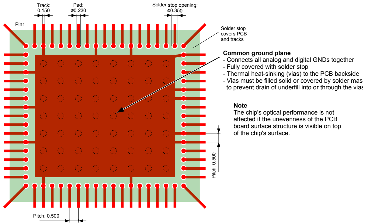
Figure 12: Recommended PCB layout (all measures in mm)
