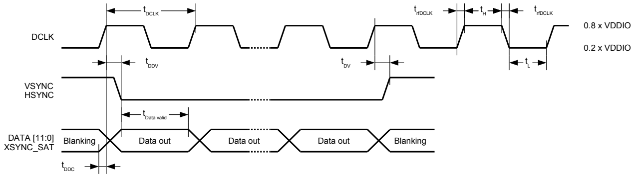
Figure 26: Detailed TCMI timing
