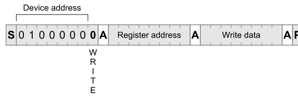
Figure 67: Single-byte Write access through I 2 C
