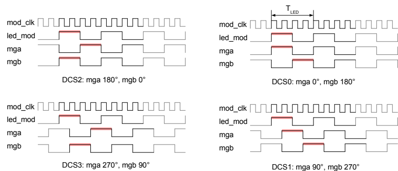
Figure 48: 4 DCS modulation/demodulation waveforms
