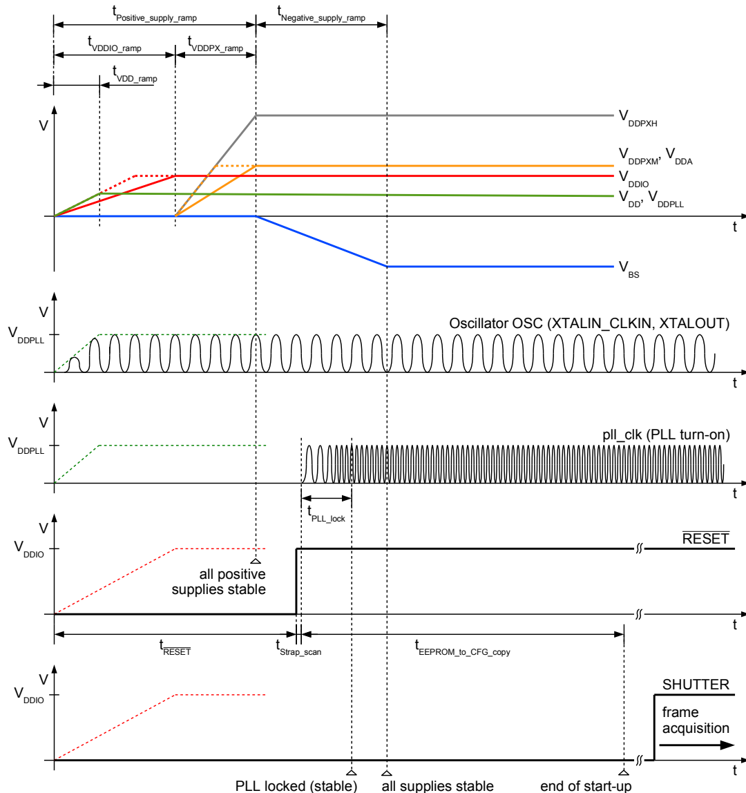
Figure 20: Power-up and reset sequence
