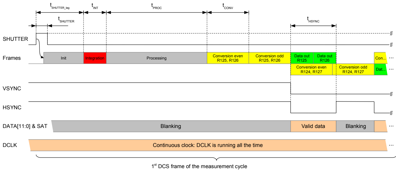
Figure 28: Frame timing: Start 1 st DCS frame
