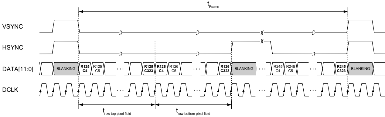
Figure 30: 12-bit mode data readout
