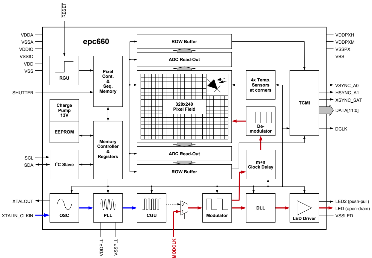
Figure 19: The MODCLK signal flow (red marked)
