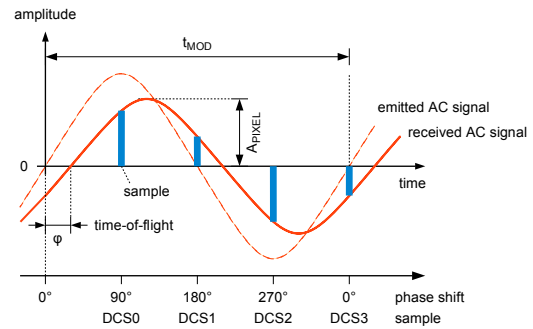
Figure 51: Sampling of the received waveform
