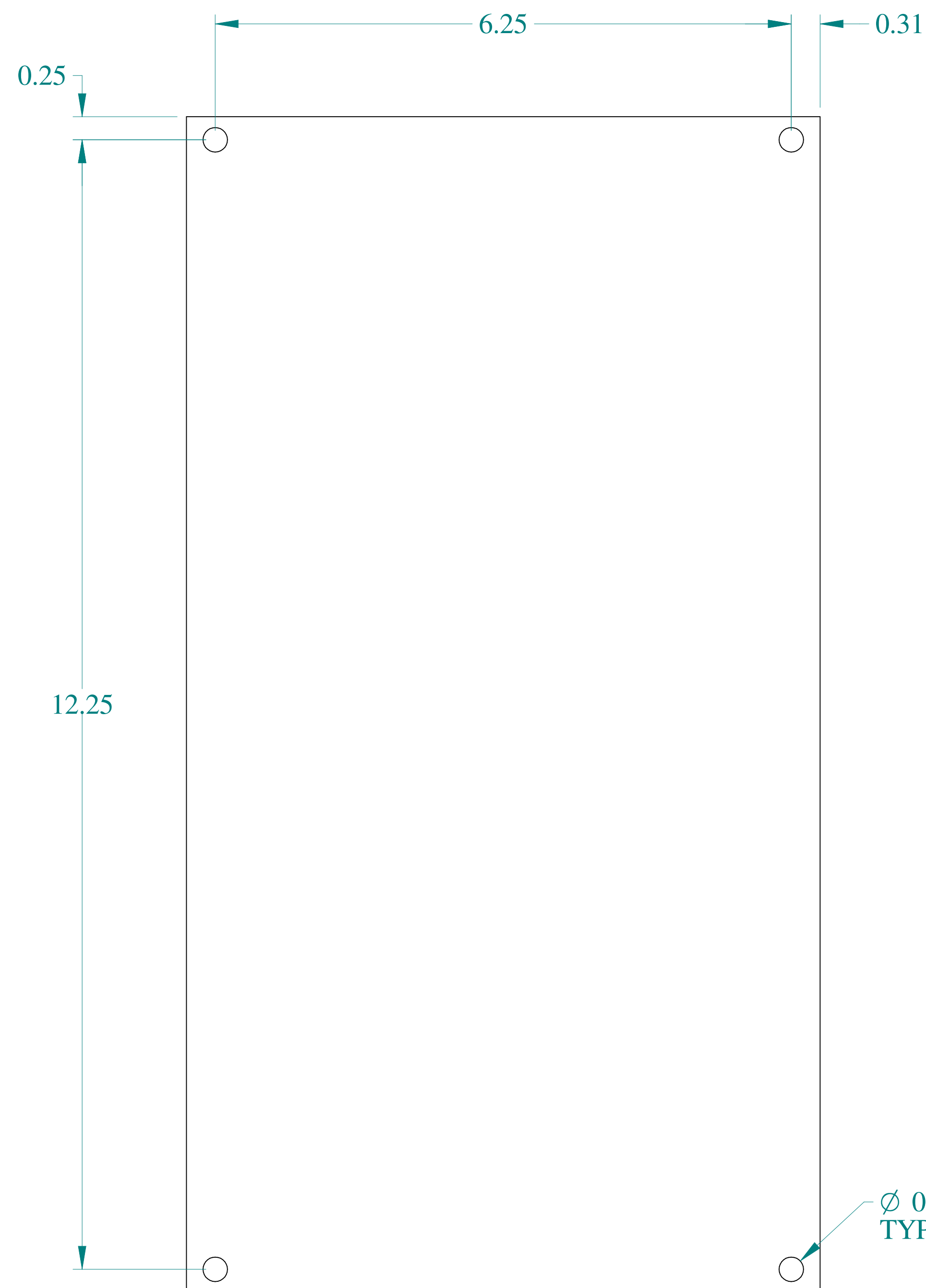
FRONT VIEW
