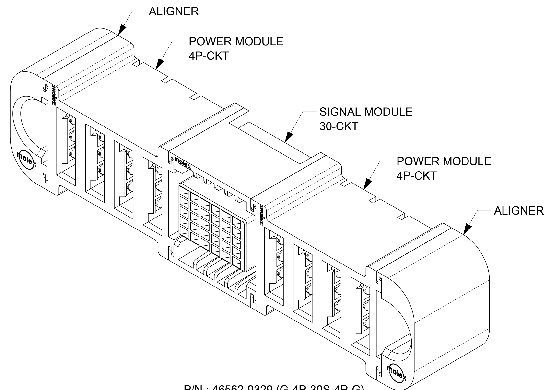
P/N : 46562-9329 (G-4P-30S-4P-G)
