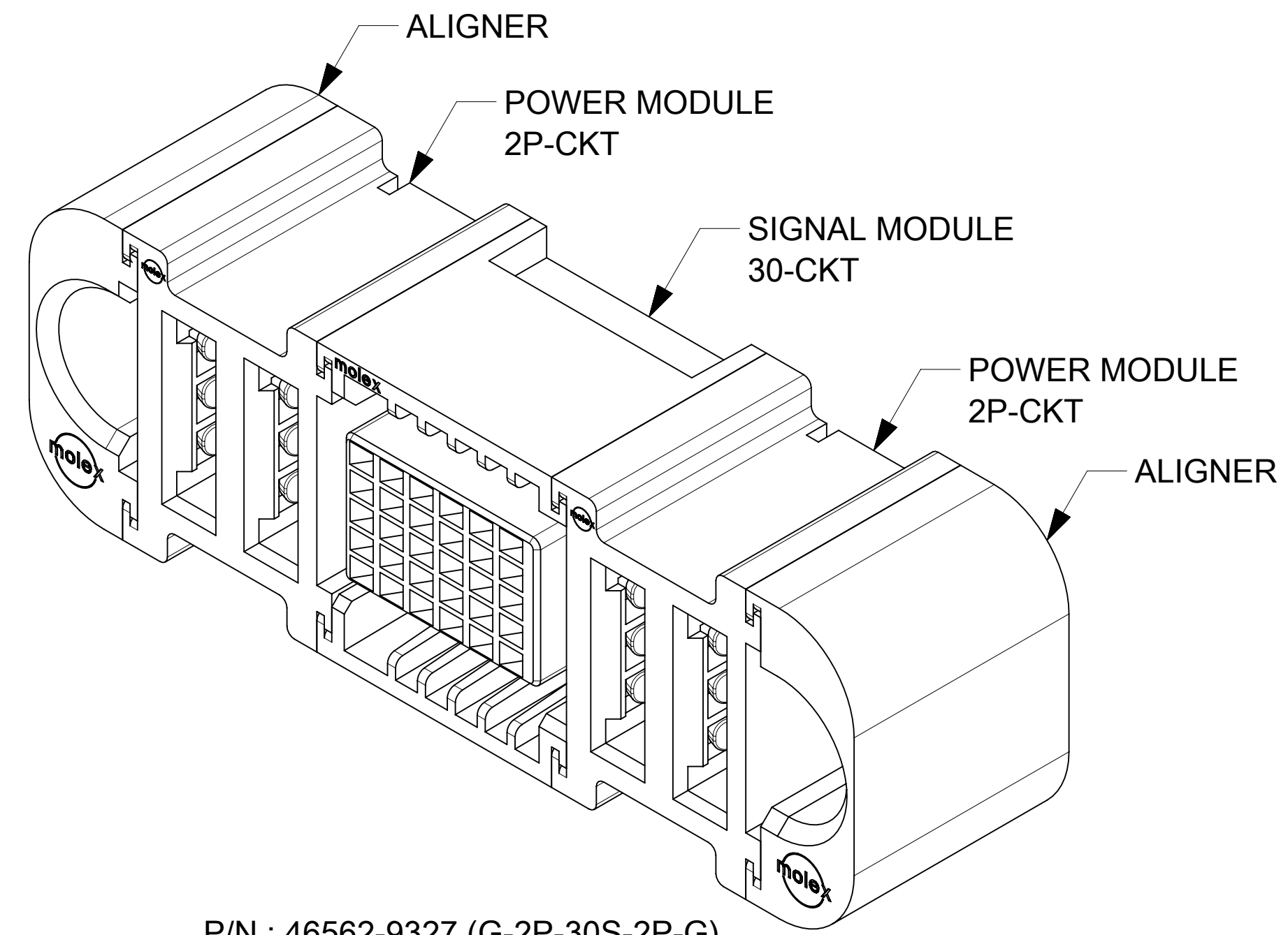
P/N : 46562-9327 (G-2P-30S-2P-G)
