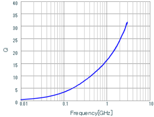
LQP02TN1N4C02 Q.
