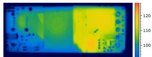
Thermal Image of module @ 48Vin, 200LFM & 55C
