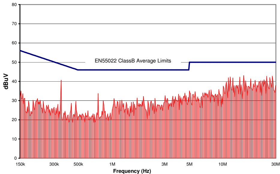
Figure 18. CPE20A36 Conducted Emissions using above specified input filter, Vin = 48V, Full Resistive Load
