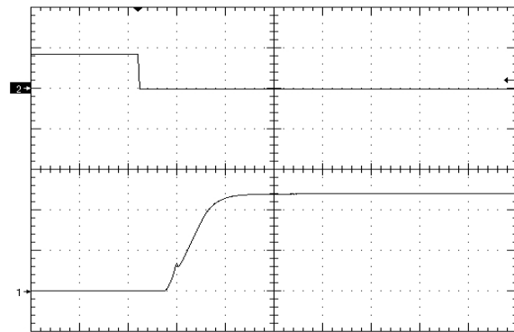
Figure 10. Startup Waveform via Enable Pin, time scale 4mS/div. Vin=Vin_nom, full load + 4700uF (neg. enable.) Ch1=2V/div,Ch2=5V/div
