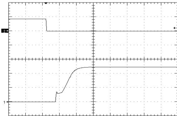
Figure 9. Startup Waveform via Enable Pin, time scale 4mS/div. Vin=Vin_nom, No Load (negative enable.) Ch1=2V/div,Ch2=5V/div
