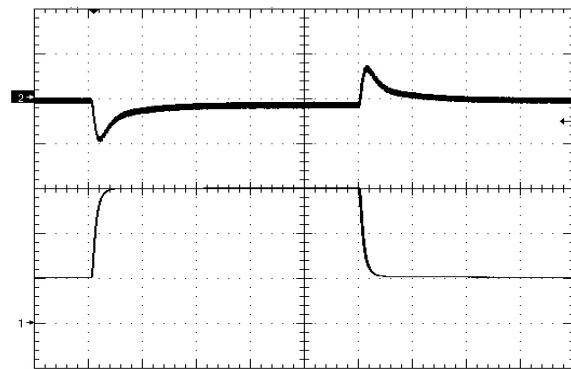
Figure 12. Load Transient Response (100mV/div), di/dt=0.1A/uS, 25% - 75% - 25% of full load, +4700uF, time scale: 200uS/div
