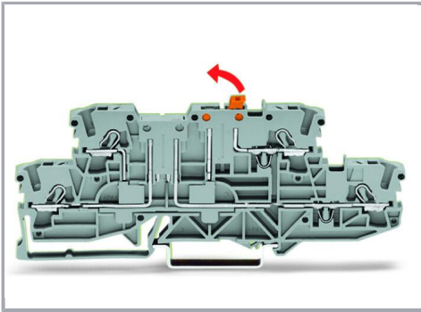
Double-deck disconnect terminal block (2002-2971)
