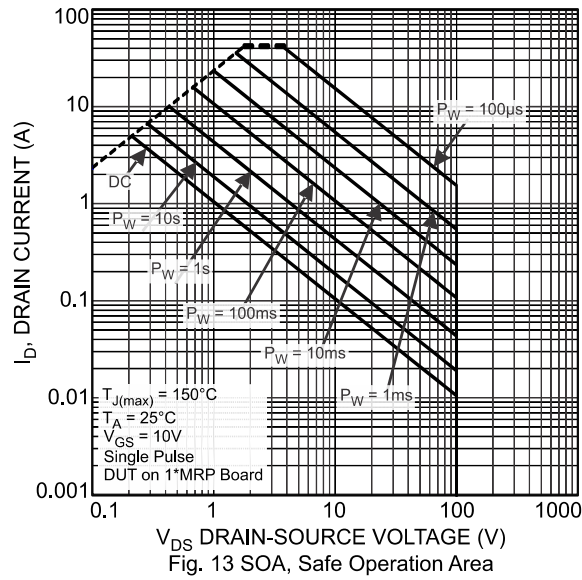
Fig. 13 SOA, Safe Operation Area
