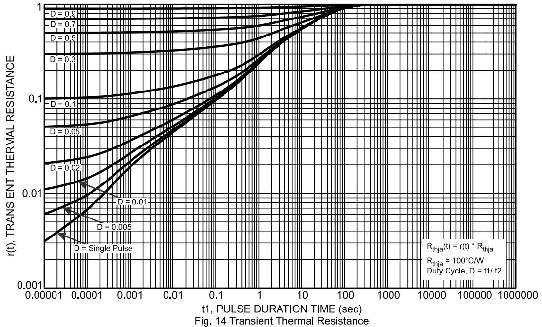
Fig. 14 Transient Thermal Resistance
