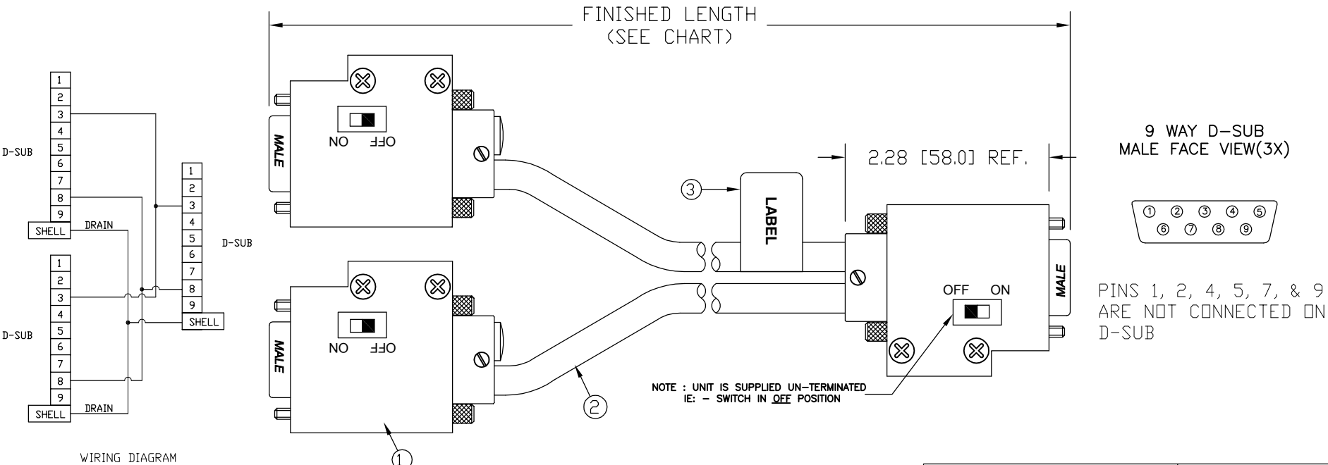
WIRING DIAGRAM
