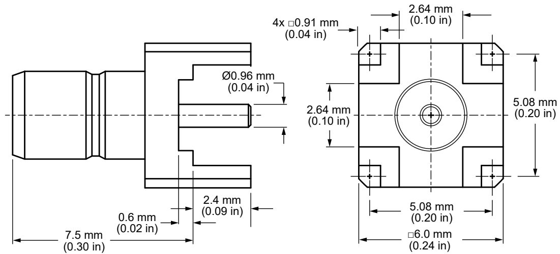
Figure 1. Product Dimensions for the CON SMA024-G Connector
