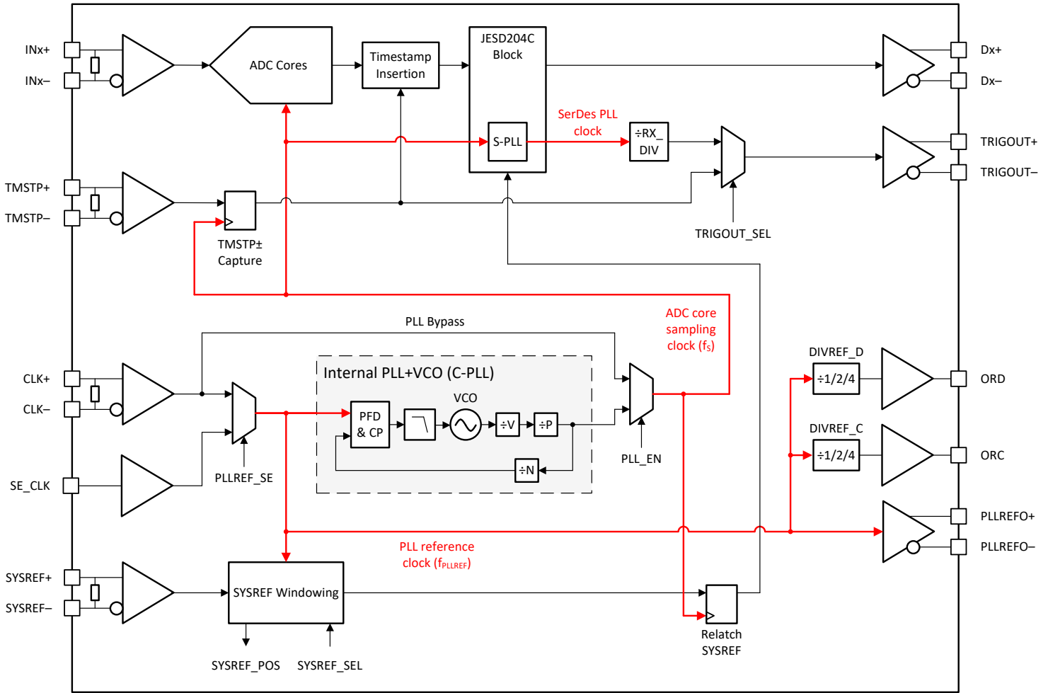
Figure 9-5. Clocking Subsystem
