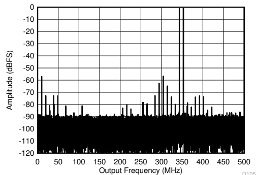
Figure 8-70. Two Tone FFT at 1798MHz
