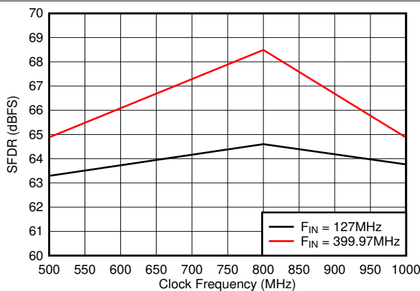
Figure 8-27. SFDR vs Sample Rate
