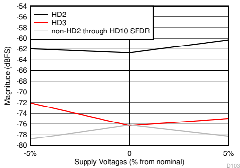
All supplies changed together, low power mode, F_S = 1000\text{MSPS}
