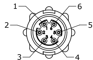
FACE VIEW 18980-6SG-5XX 6 POSITION B-KEY
