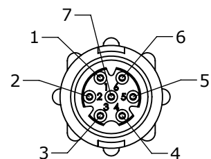
FACE VIEW 18980-7SG-5XX 7 POSITION A-KEY
