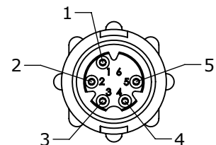
FACE VIEW 18980-5SG-5XX 5 POSITION A-KEY
