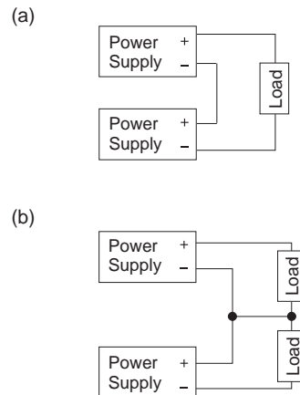
Fig. 5.1 Examples of series operation
