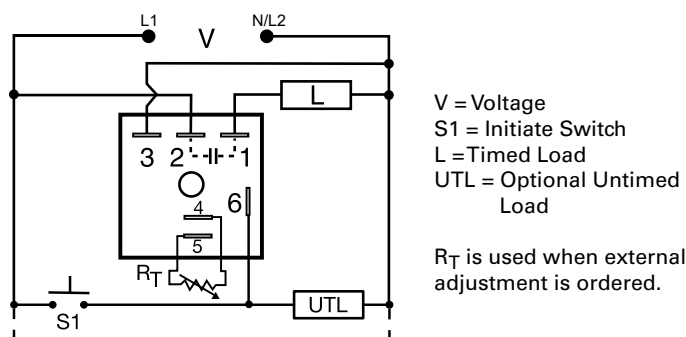
For dimensional drawing see: Appendix, page 512, Figure 16.
