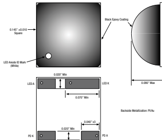
Fig. 8 4-Lead Surface Mounted Ceramic Chip Carrier
