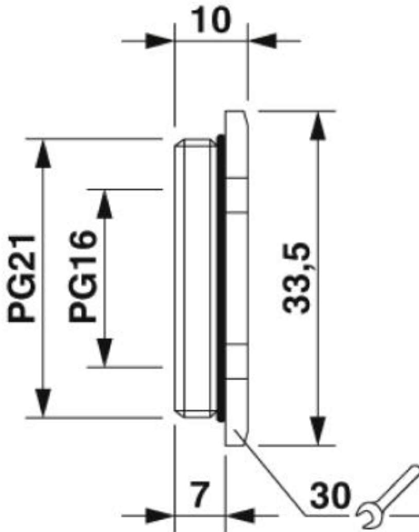
Dimensional drawing
