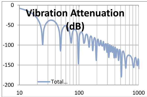
Attenuation vs. Vibration Frequency Fclk = 12.5kHz
