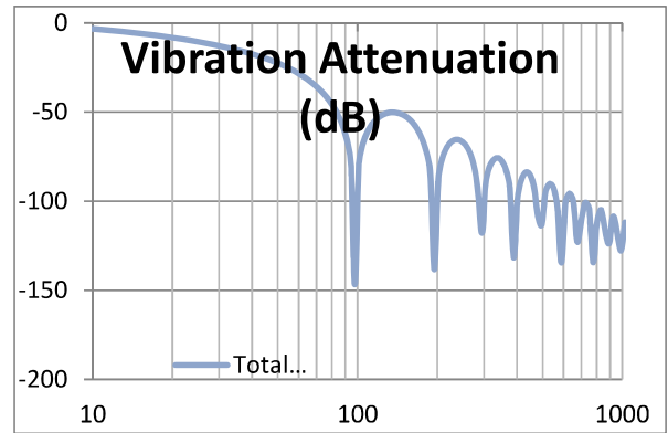
Attenuation vs. Vibration Frequency Fclk = 50kHz
