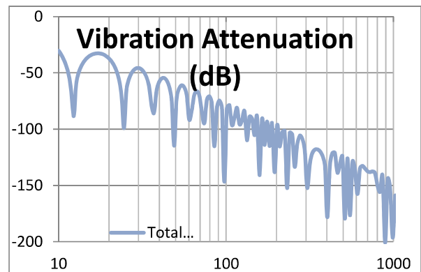
Attenuation vs. Vibration Frequency Fclk = 6.25kHz
