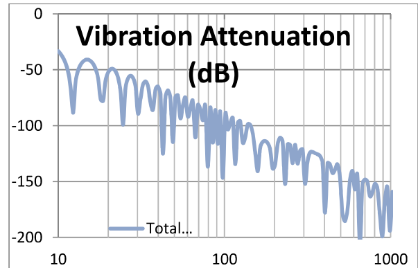
Attenuation vs. Vibration Frequency Fclk = 3.125kHz
