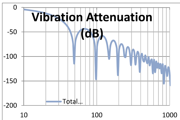
Attenuation vs. Vibration Frequency Fclk = 25kHz
