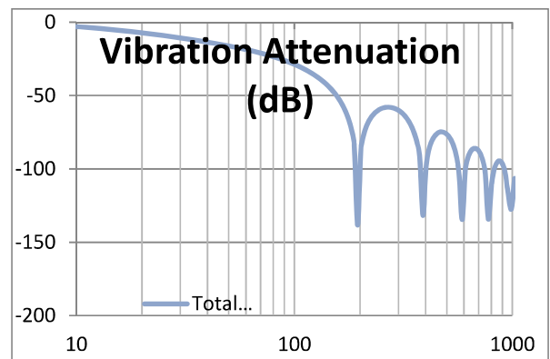
Attenuation vs. Vibration Frequency Fclk = 100kHz
