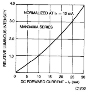
Fig. 2. Relative Luminous Intensity vs. DC Forward Current
