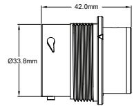
Size 18 Receptacle (SRA) Smooth Ring Adapter
