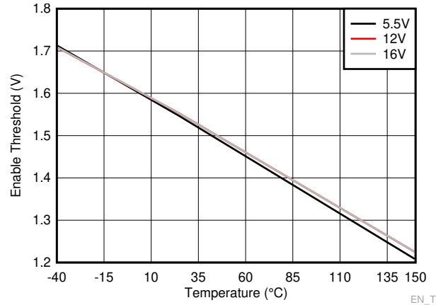
Figure 6-10. Enable Threshold
