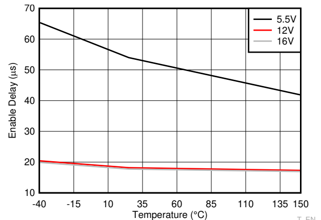
Figure 6-12. Enable Delay
