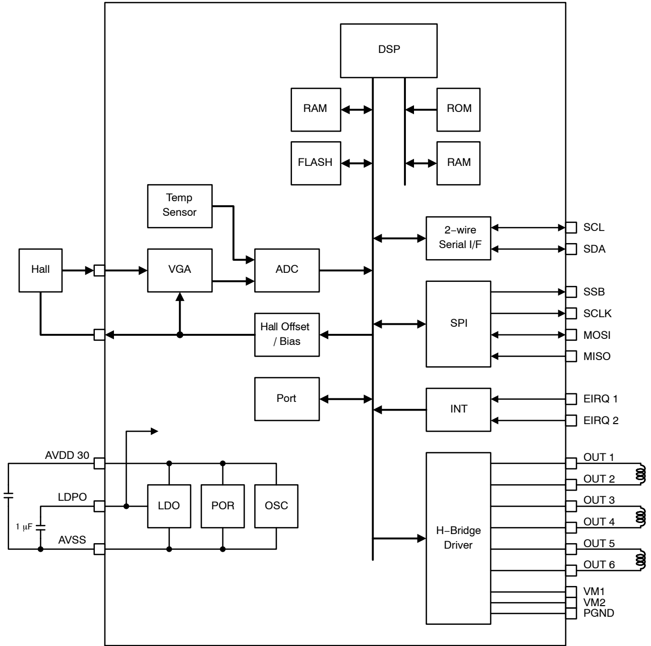
Figure 1. Block Diagram
