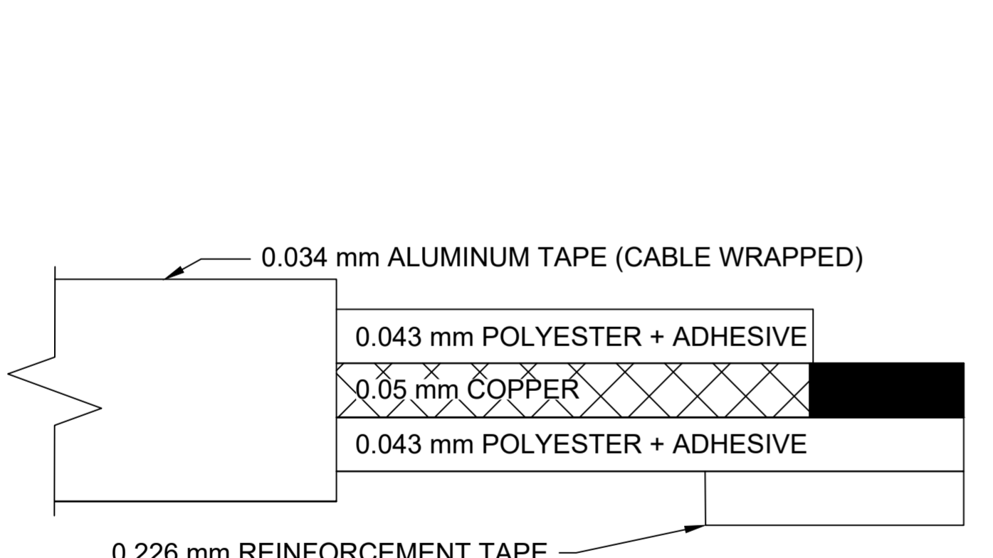
CROSS-SECTION
