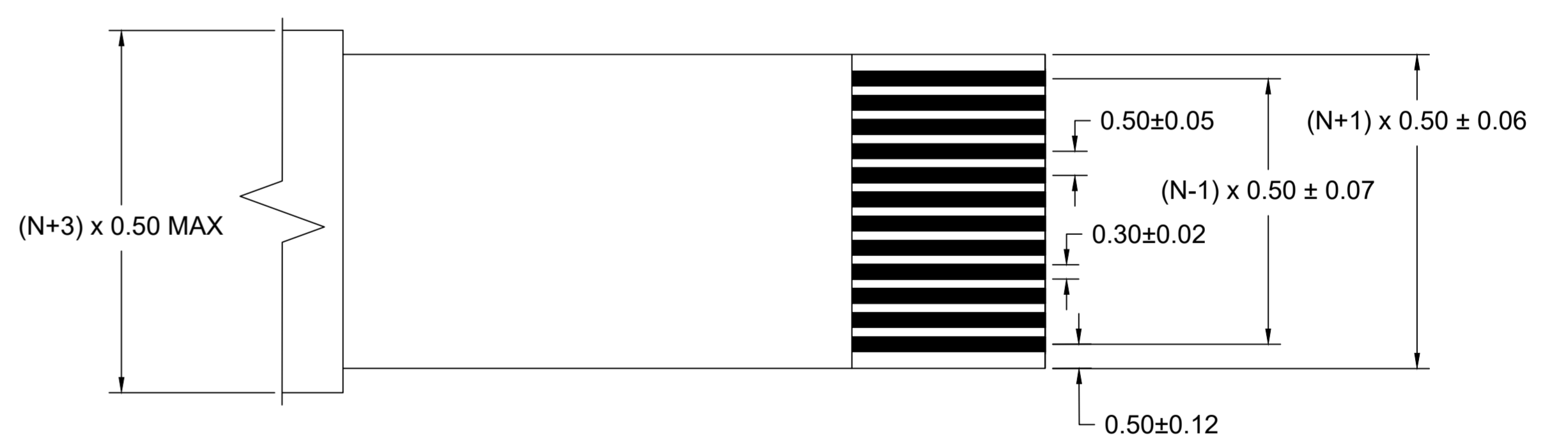
END-TAIL DIMENSIONS SCALE 10:1
