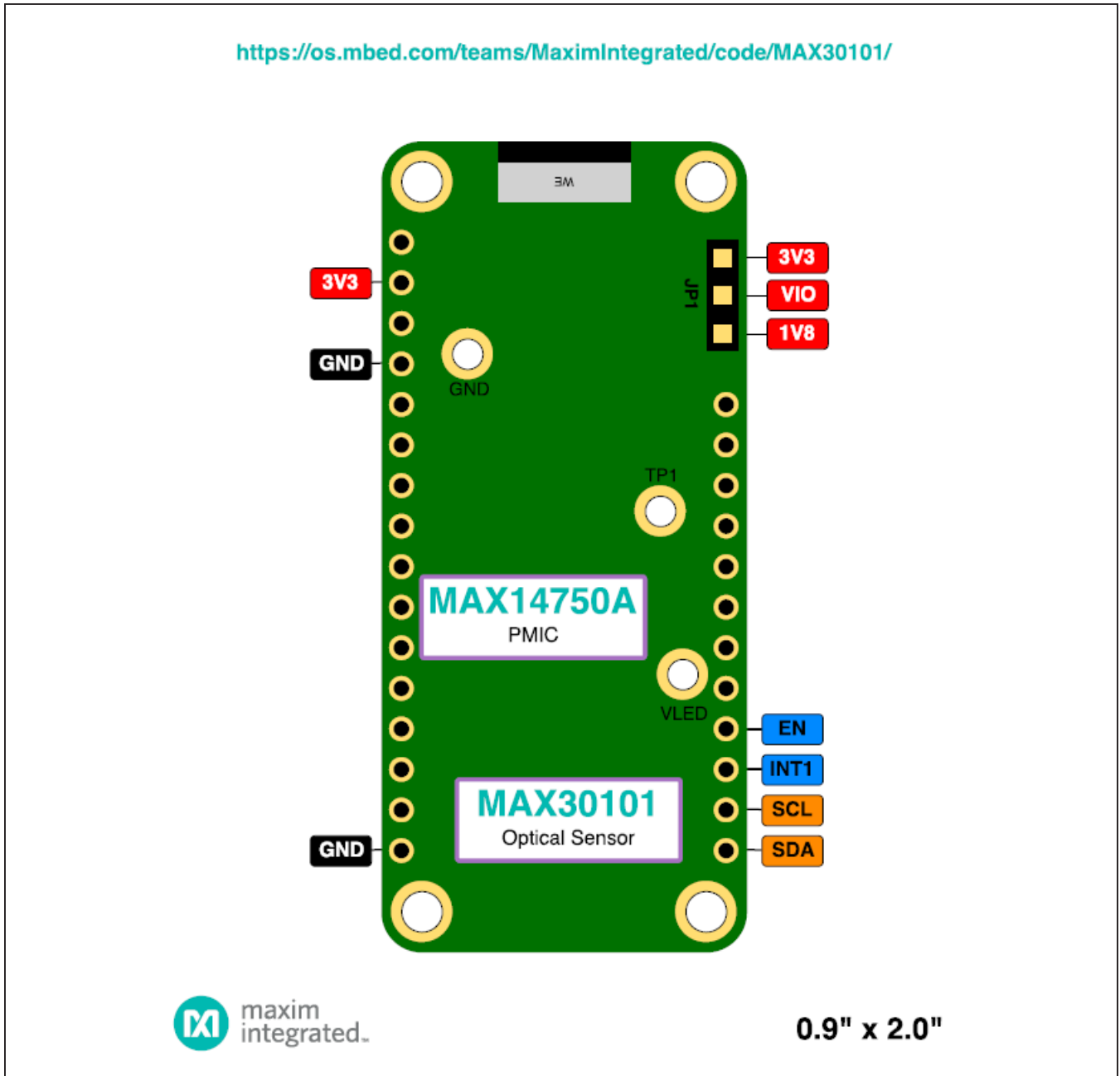
Figure 1. DIP Pinout
