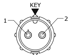
FACE VIEW 8380-2PG-5XX
