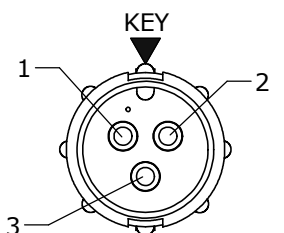
FACE VIEW 8380-3PG-5XX
