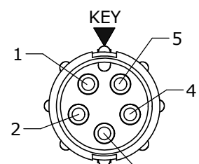
FACE VIEW 8380-5PG-5XX
