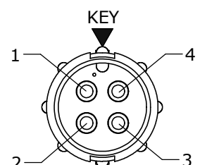
FACE VIEW 8380-4PG-5XX
