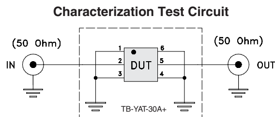
Fig 1. Block diagram of Test Circuit used for characterization, Test board TB-YAT-30A+ Conditions: Attenuation, VSWR: Pin=-10 dBm
