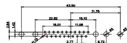
25W3 Female
