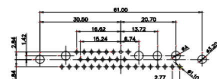
36W4 Female
