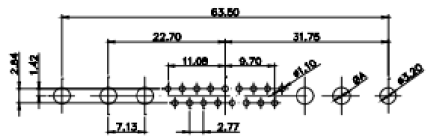
21W4 Male/Female
