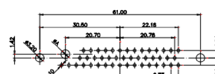
47W1 Female
