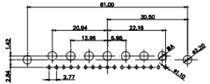
24W7 Male/Female
