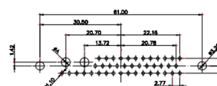
43W2 Female
