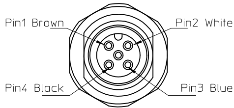
FRONT SIDE VIEW FEMALE 4 POLE
