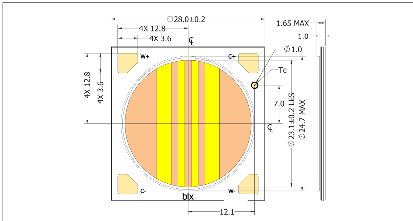
Figure 14: Drawing for Vesta Series Tunable White Gen 2 22mm Array
