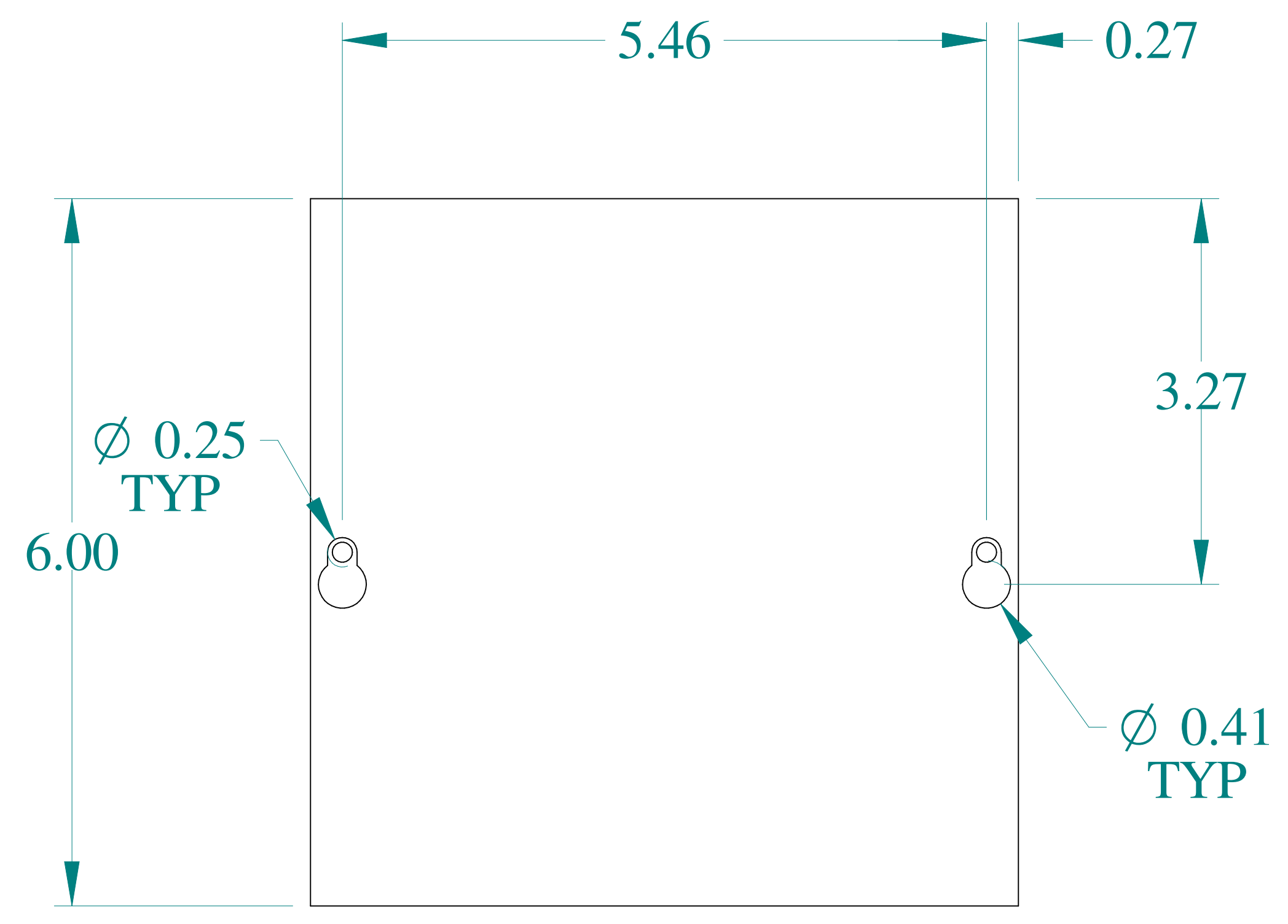
TOP VIEW
