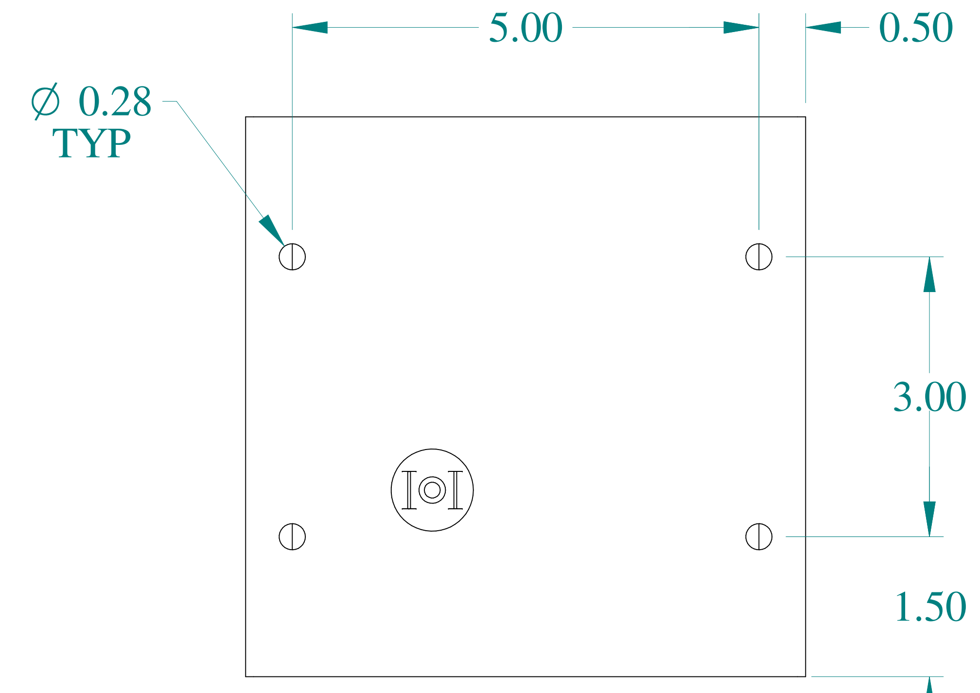
BOTTOM VIEW
