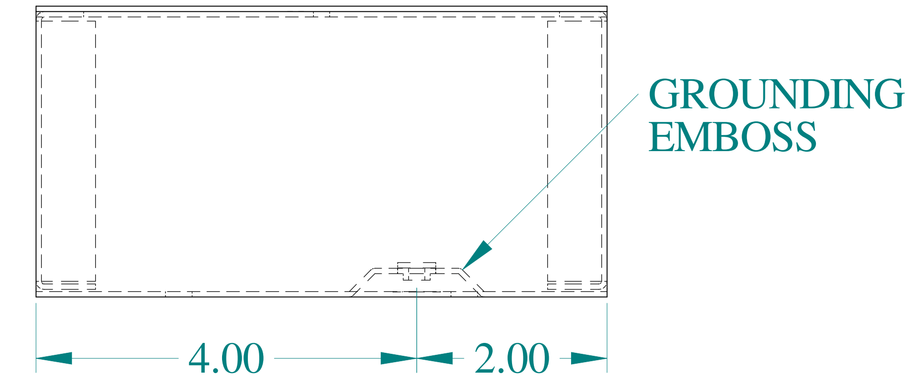
SIDE VIEW
