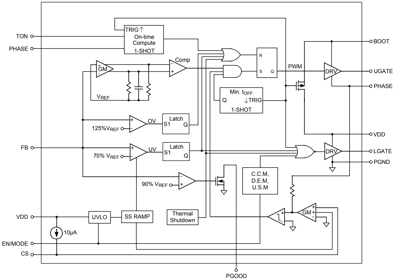
PWM Controller
