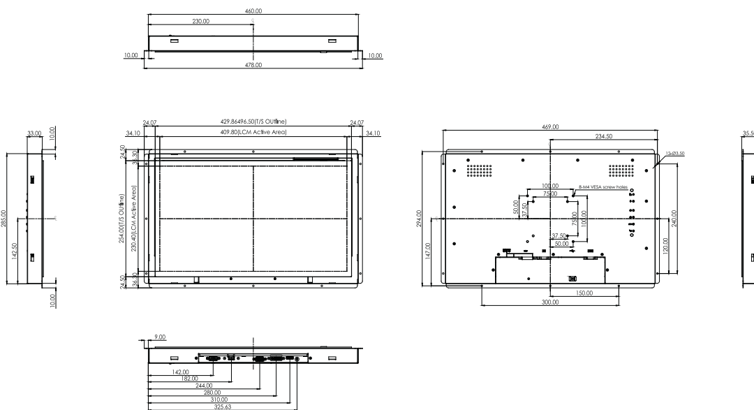
Figure 2.1 IDS-3118W Dimensions
