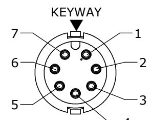
FACE VIEW ASSY: 6280-7SG-5XX
