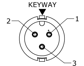
FACE VIEW ASSY: 6280-3SG-5XX
