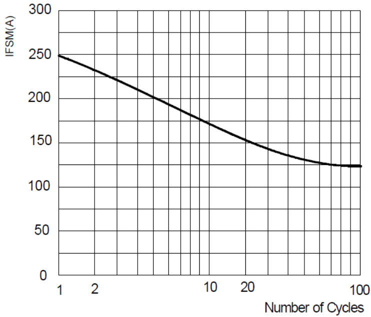
Fig3: Surge Forward Current Capadility
