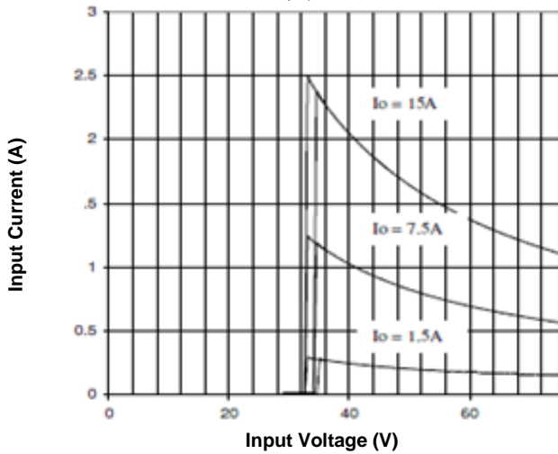
Figure 9. Input Characteristics
