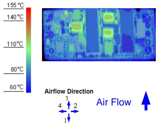
Figure 12. Thermal Image for Airflow Direction 3 (15A output, 55°C ambient, 200 LFM, typical V_{in} , open frame, socket interface)
