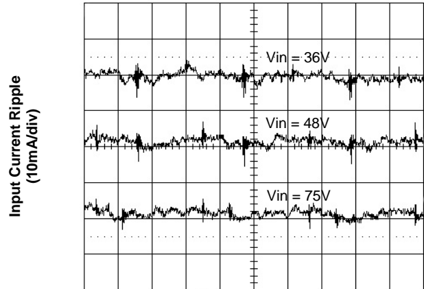
Figure 6. Input Reflected Ripple Current at Full Load
