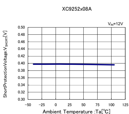
(16) Short Protection Threshold Voltage vs. Temperature
