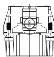
TYPE 3, T2049102101-000, LASER WITHOUT LOGO 类型 3, T2049102101-000, 激光标识不带 LOGO
