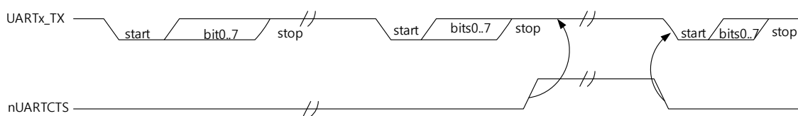
Figure 51. CTS Functional Timing
