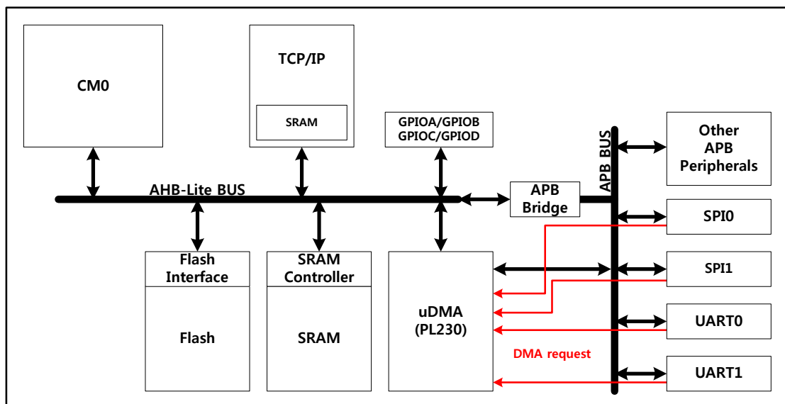
Figure 17. DMA Block diagram
