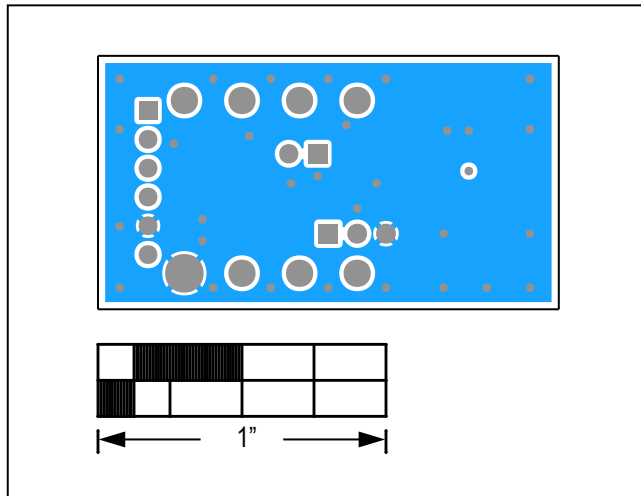
MAX1240 EV Kit—Bottom
