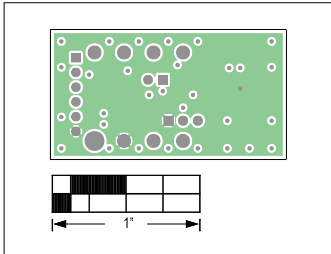
MAX1240 EV Kit—Layer 3
