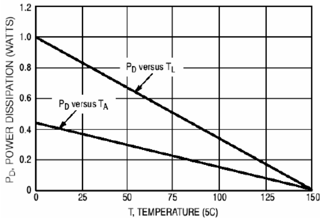
Fig 3. Steady State Power Derating
