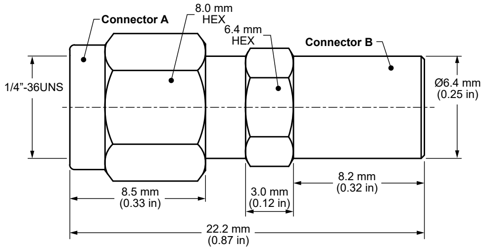
Figure 1. Product Dimensions for the ADP-SMAM-SMBM-G Adapter
