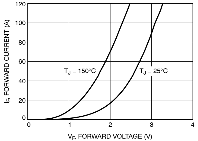
Figure 5. Typical Diode Forward Characteristics
