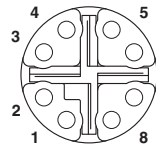
Assignment of the LAN female connector
