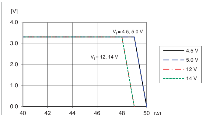
Output voltage vs. load current at T_{pj} = +25\text{ }^\circ\text{C} , V_0 = 3.3\text{ V} . Note: Output enters hiccup mode at current limit.
