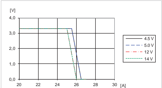
Output voltage vs. load current at T_{P1} = +25 °C , V_O = 3.3 V . Output enters hiccup mode at current limit.
