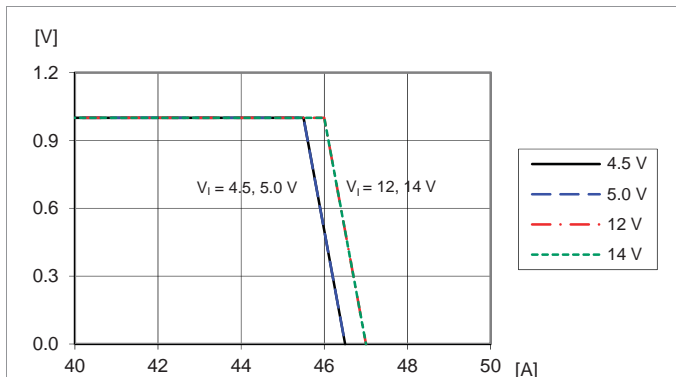
Output voltage vs. load current at T_{pj} = +25\text{ }^\circ\text{C} , V_0 = 1.0\text{ V} . Note: Output enters hiccup mode at current limit.
